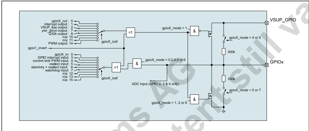
Figure 22. GPIO block diagram
