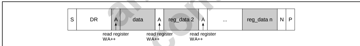
Figure 29. Current Address Read
