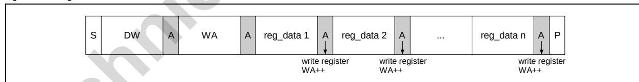
Figure 26. Page Write
