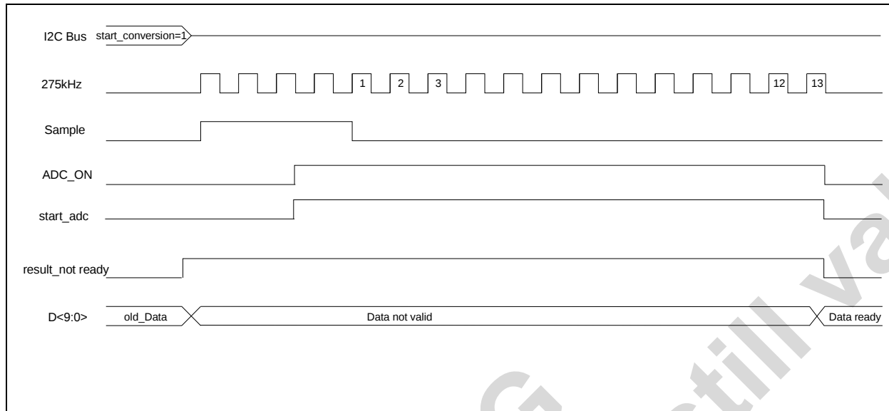
Figure 24. ADC Timing-diagram
