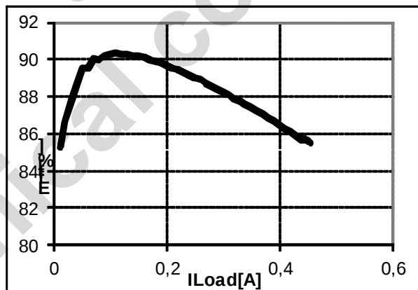
8.6.7 Step-Up DC/DC Controller Efficiency vs. Output Current; V SUP = 3.8V, T A = +25°C
