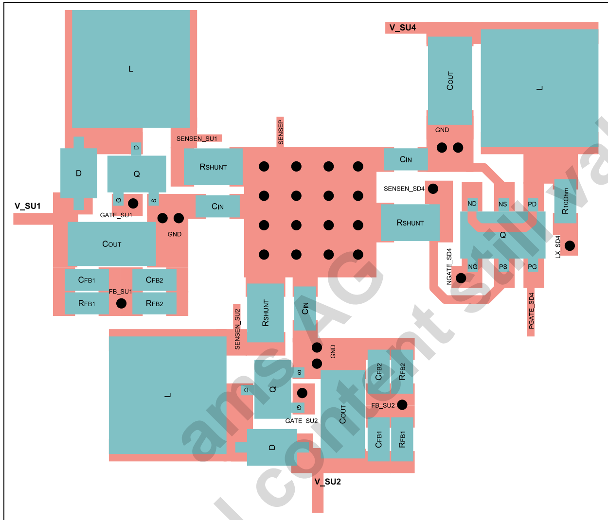
Figure 32. PCB Layout Recommendation for SU1, SU2, SD4
