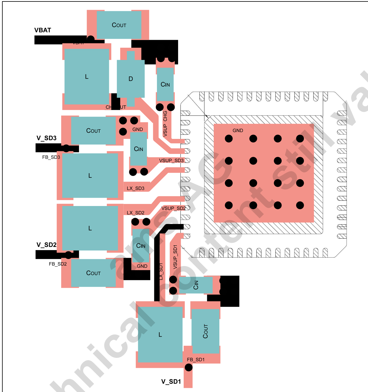
Figure 31. PCB Layout Recommendation for SD1, SD2, SD3 and Switched Mode Charger
