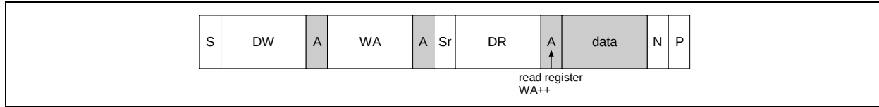
Figure 27. Random Read
