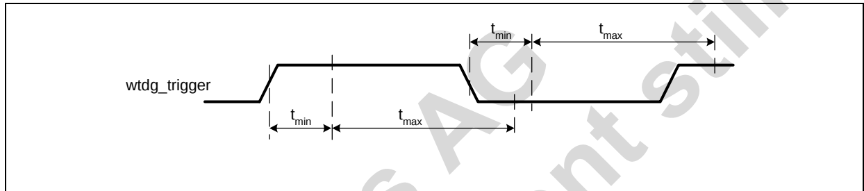
Figure 23. Watchdog timing diagram
