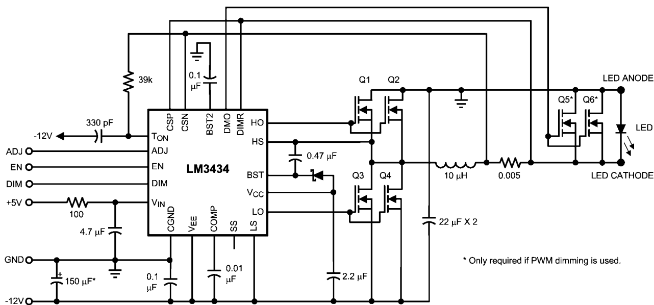
FIGURE 2. Up to 20A Output Application Circuit
