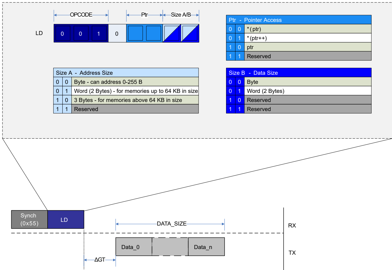
Figure 33-10. LD Instruction Operation
