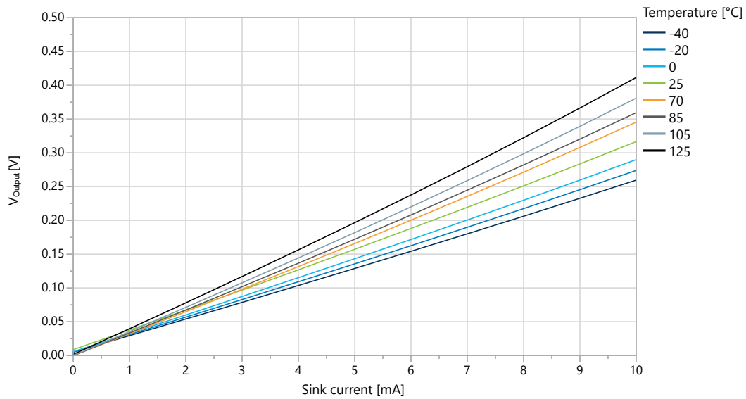
Figure 37-22. I/O Pin Output Voltage vs. Sink Current ( V_{DD} = 3.0V )
