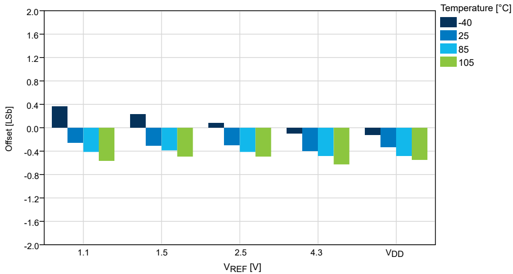
Figure 37-51. Offset Error vs. V_{REF} ( V_{DD} = 5.0V , f_{ADC} = 115 kps), REFSEL = Internal Reference
