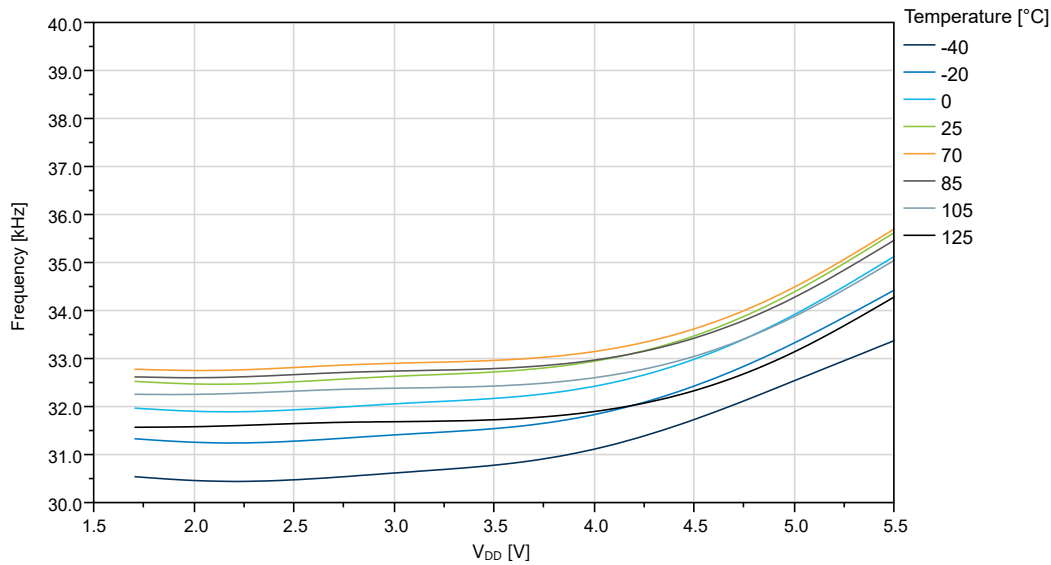
Figure 37-66. OSCULP32K Internal Oscillator Frequency vs. V_{DD}
