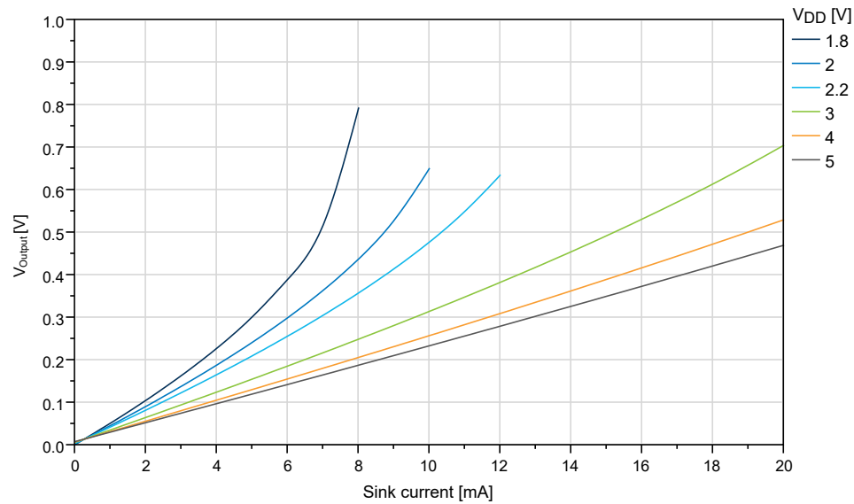
Figure 37-24. I/O Pin Output Voltage vs. Sink Current ( T = 25^{\circ}C )
