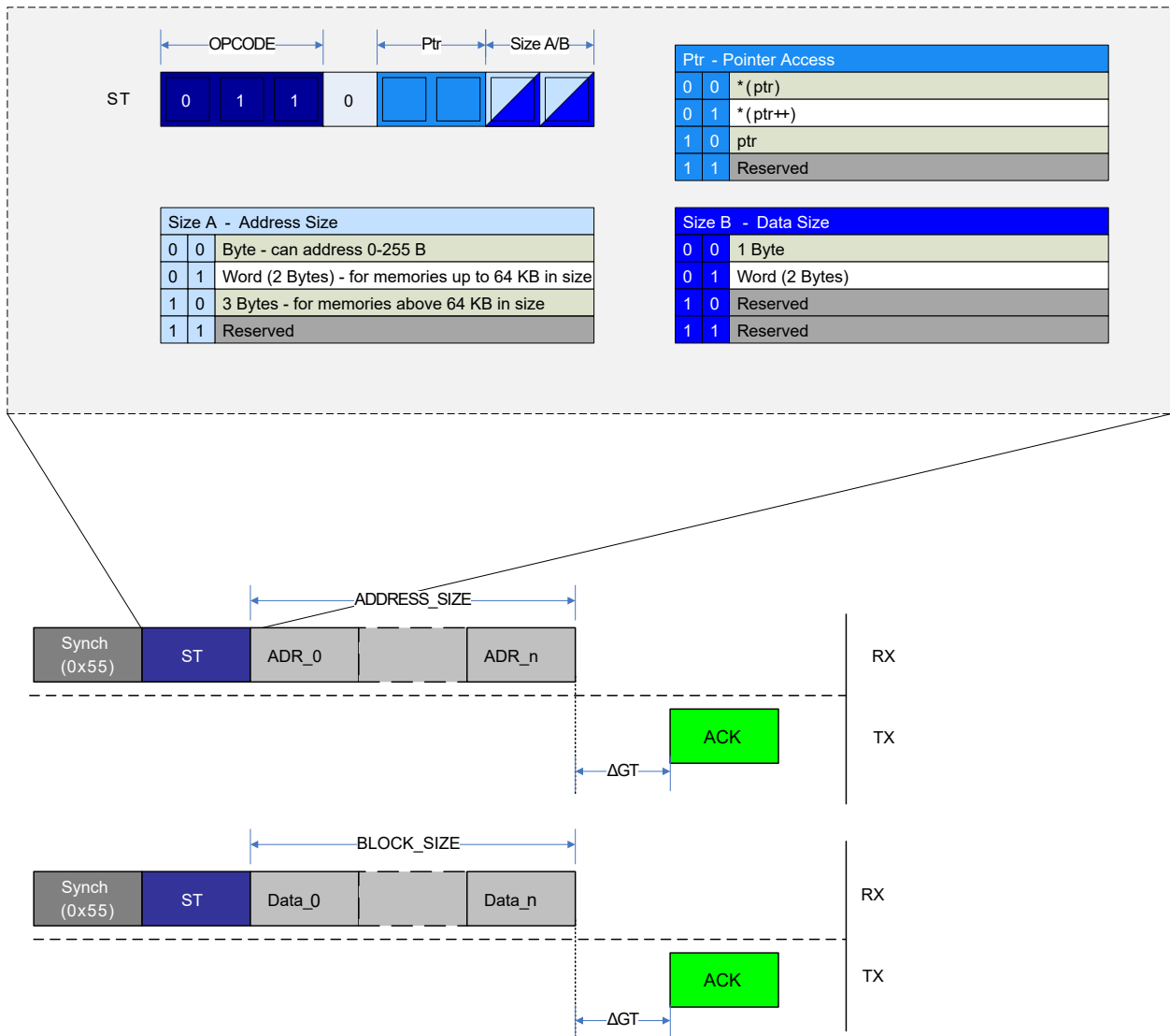
Figure 33-11. ST Instruction Operation
