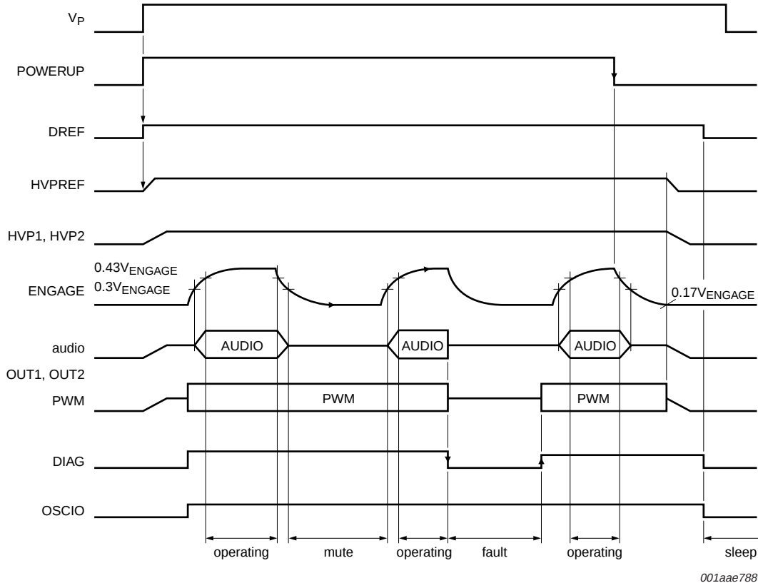
Fig 3. Start-up sequence
