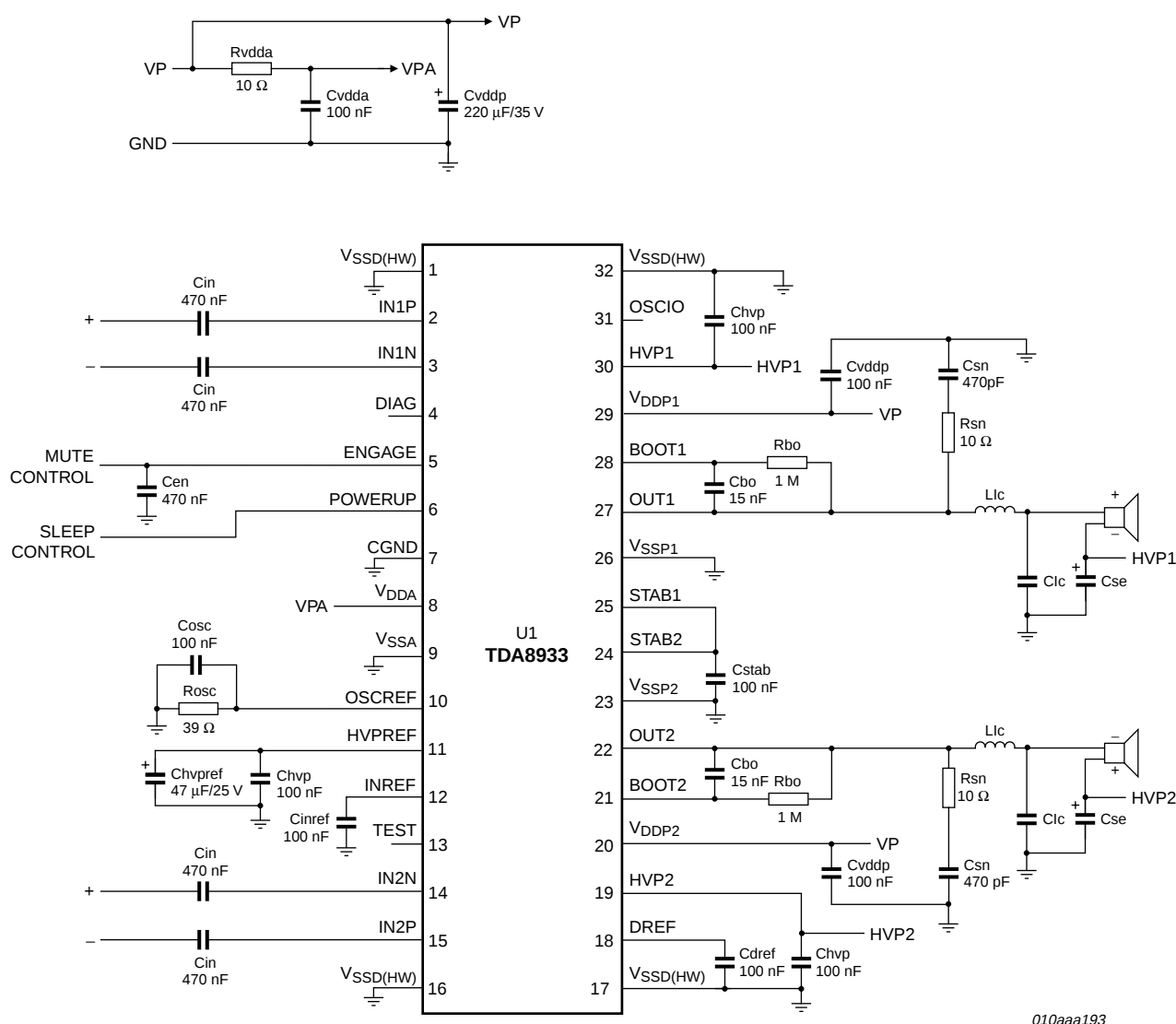
Fig 39. Typical simplified application diagram for 2 × SE (asymmetrical supply)
