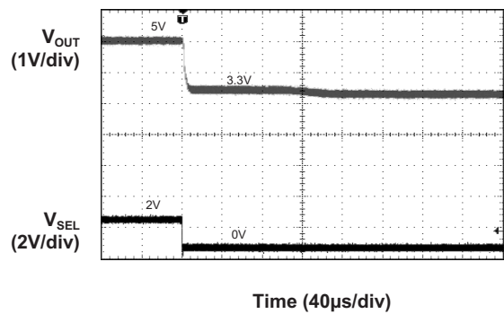
5V to 3.3V Transition Response ( I_{OUT} = 500mA , C_{OUT} = 10μF )
