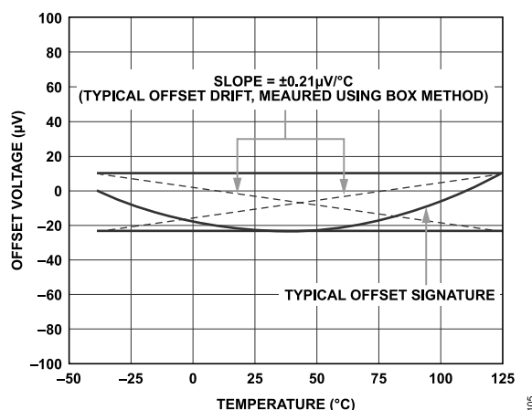
Figure 56. Box Method
