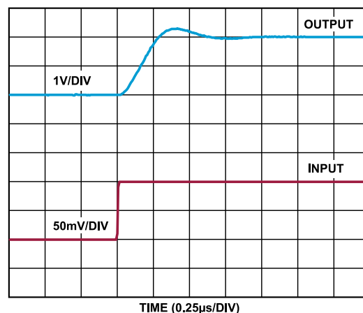
Figure 20. Rise Time, V_S = 5\text{ V}
