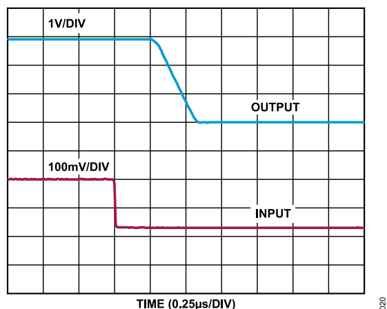
Figure 25. Differential Overload Recovery, Falling, V_S = 2.9\text{ V}
