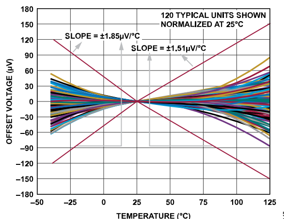
Figure 57. Bowtie Method
