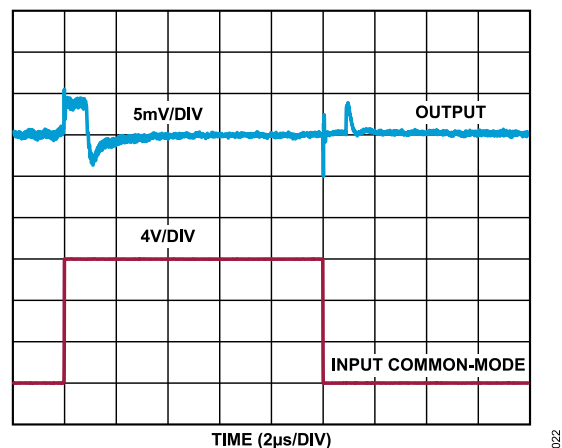
Figure 9. Input Common-Mode Step Response (0 V to 12 V), V_S = 5 V, Inputs Shorted
