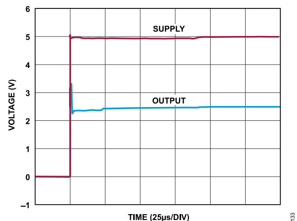
Figure 34. Start-Up Response
