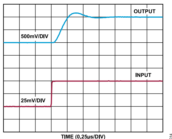
Figure 19. Rise Time, V_S = 2.9\text{ V}
