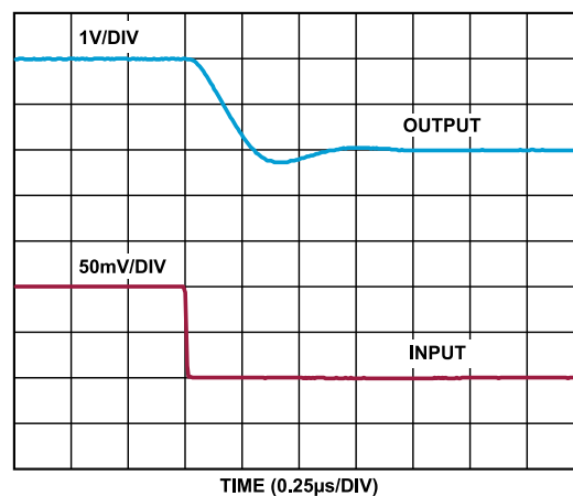
Figure 22. Fall Time, V_S = 5\text{ V}
