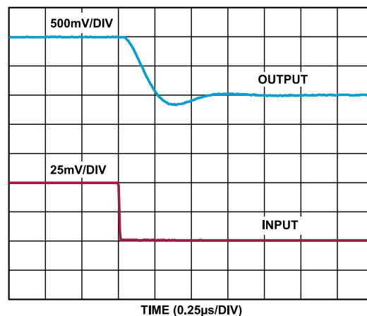
Figure 21. Fall Time, V_S = 2.9\text{ V}
