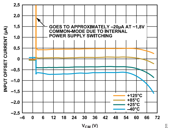
Figure 16. Input Offset Current vs. V_{CM} at Various Temperatures
