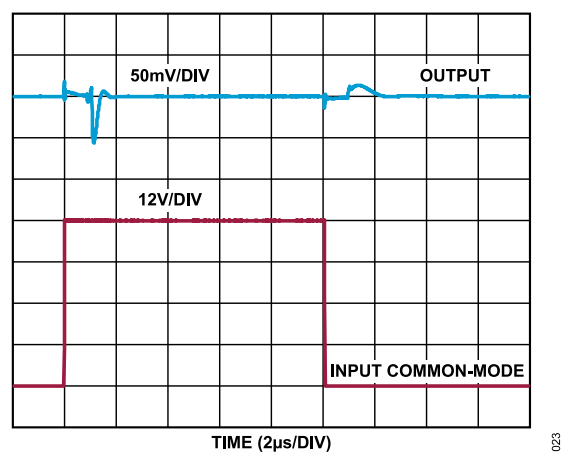
Figure 10. Input Common-Mode Step Response (0 V to 48 V), V_S = 5 V, Inputs Shorted
