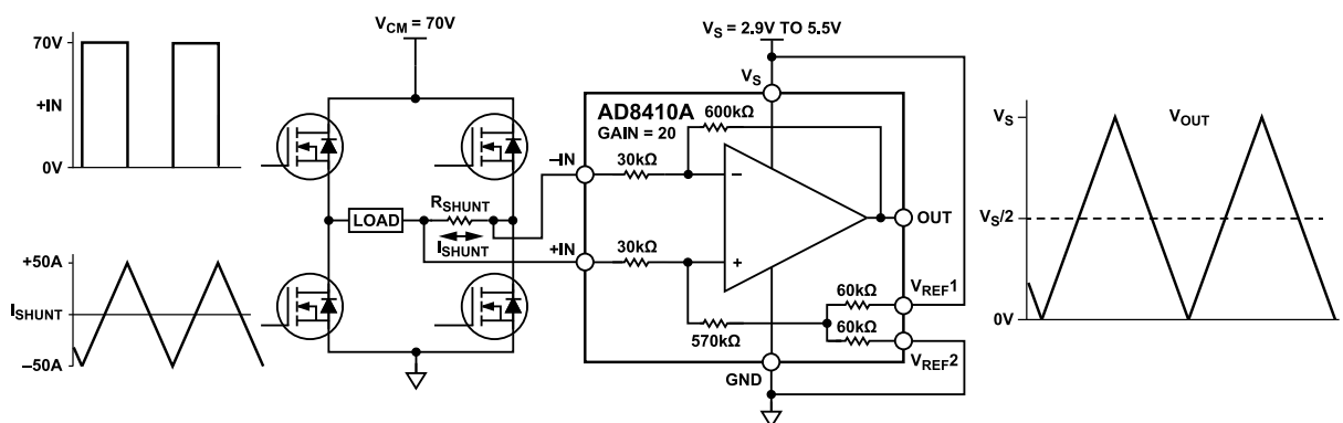
Figure 47. Typical Application
