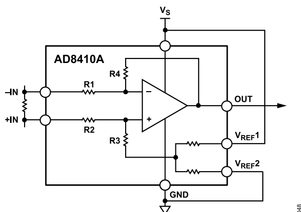
Figure 53. Split Supply
