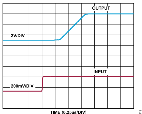
Figure 24. Differential Overload Recovery, Rising, V_S = 5\text{ V}
