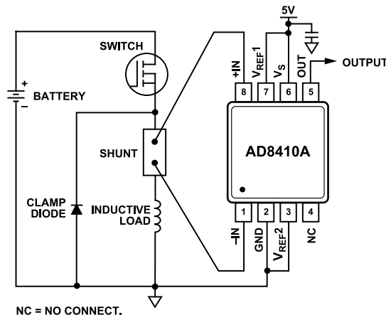
Figure 61. High-Side Switch
