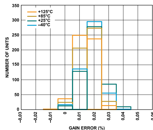
Figure 45. Gain Error Distribution
