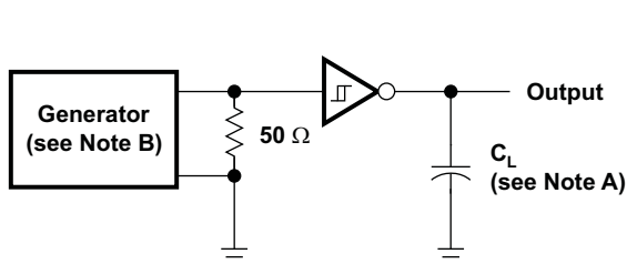
TEST CIRCUIT
