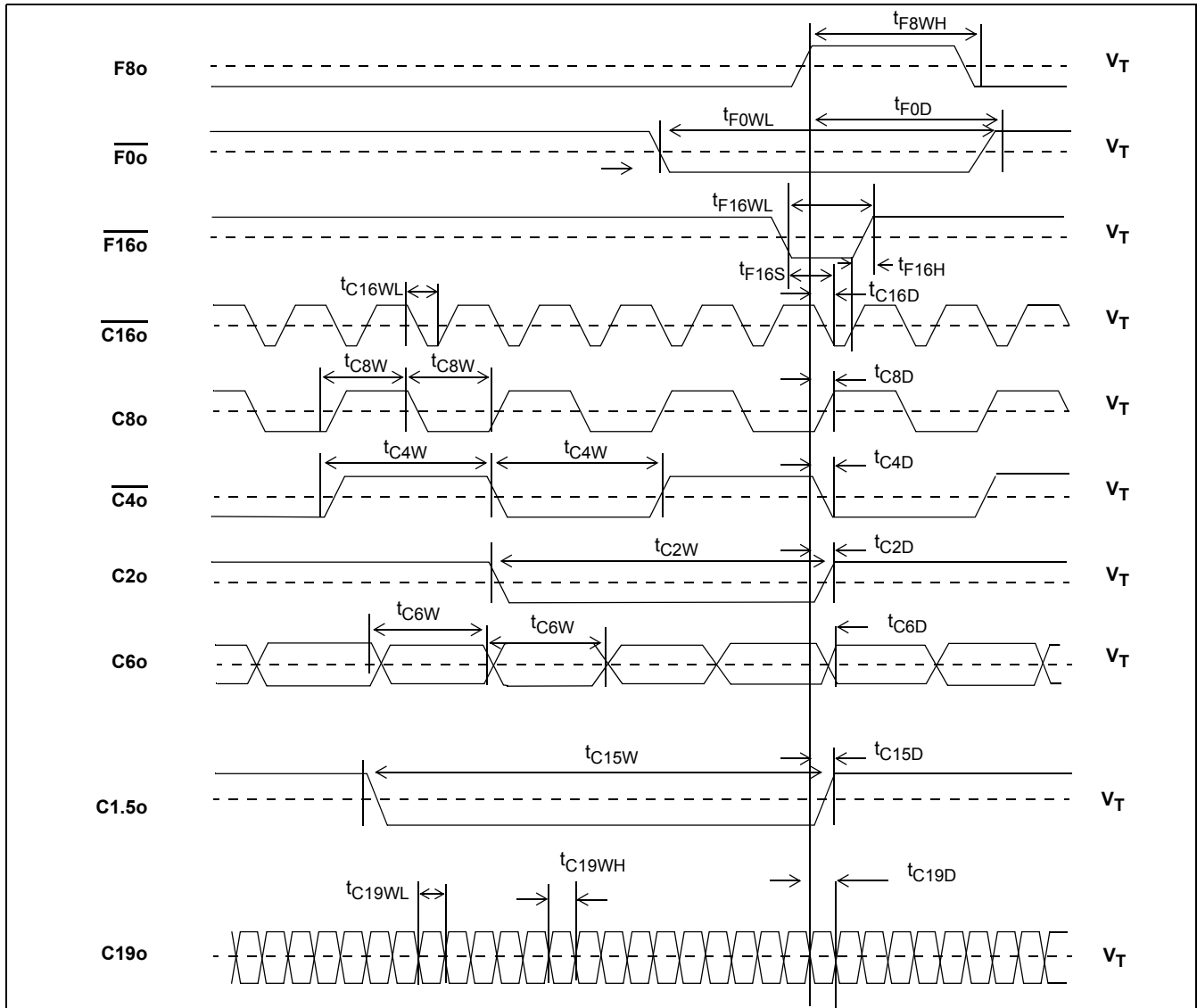
Figure 10 - Output Timing 1
