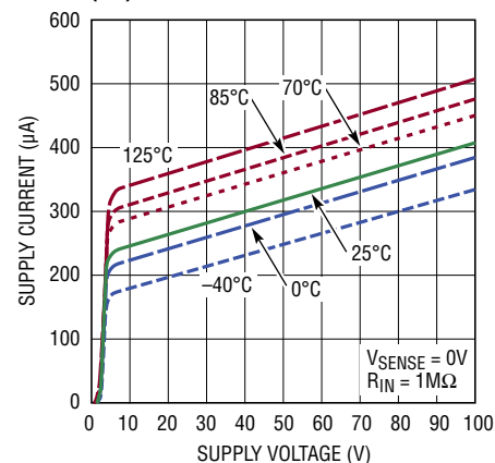
Supply Current vs Supply Voltage ( V^+ )
