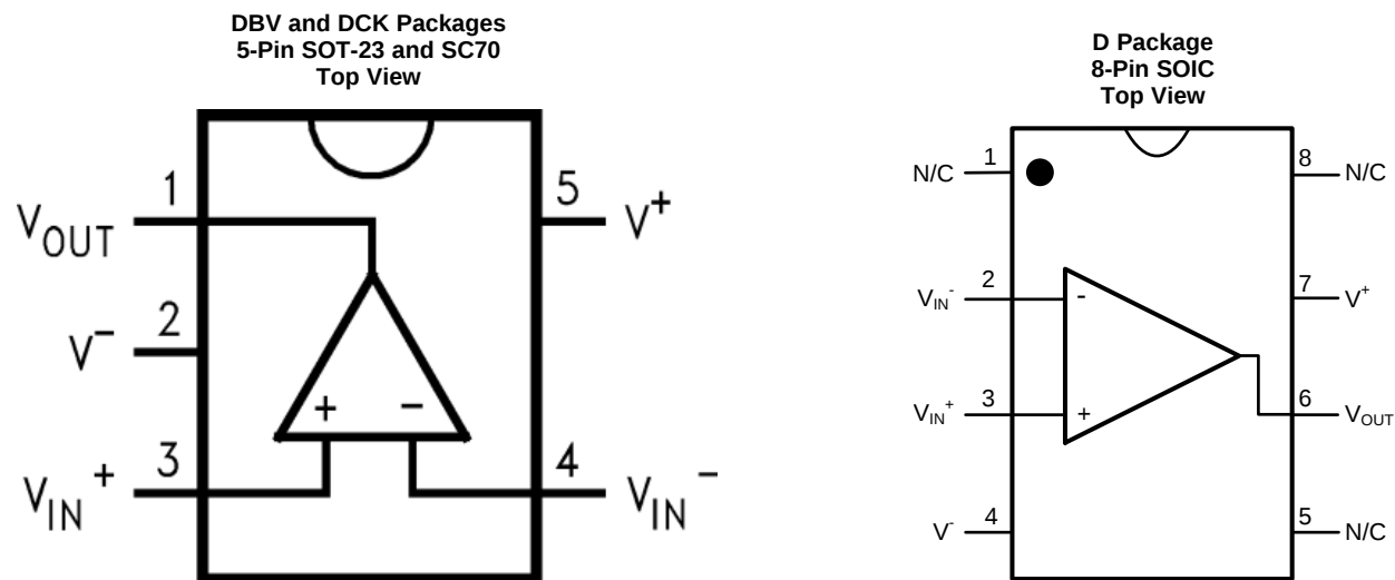
Pin Functions
