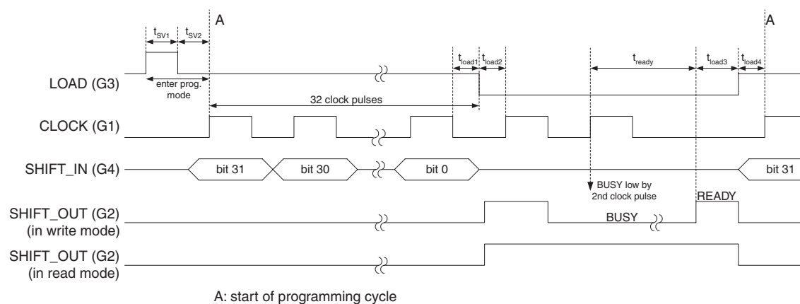
Figure 30: Programming Protocol 16
