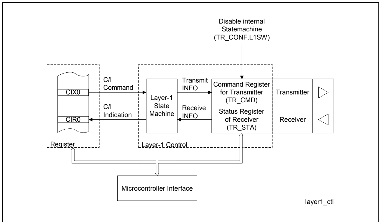
Figure 35 Layer-1 Control
