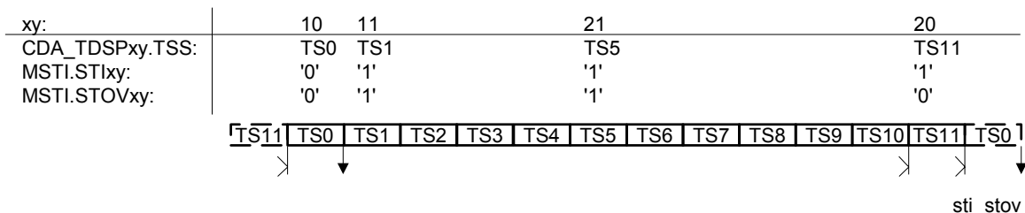
Figure 17 Examples for the Synchronous Transfer Interrupt Control with one enabled STIxy
