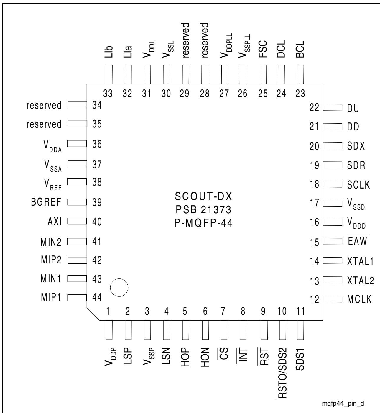
Figure 1 Pin Configuration
