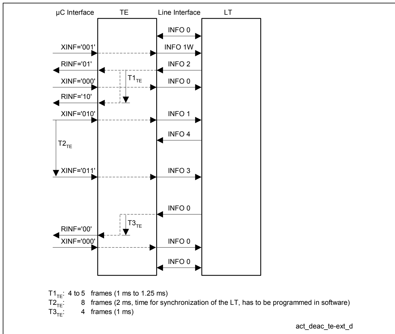
Figure 40 Example of Activation/Deactivation initiated by the Terminal (TE). Activation/Deactivation completely under software control
