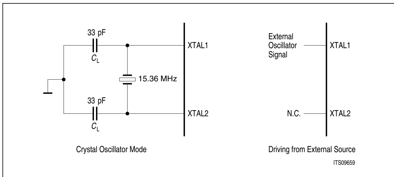
Figure 77 Oscillator Circuit
