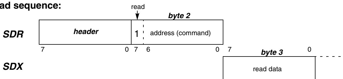
Figure 8 Serial Command Structure
