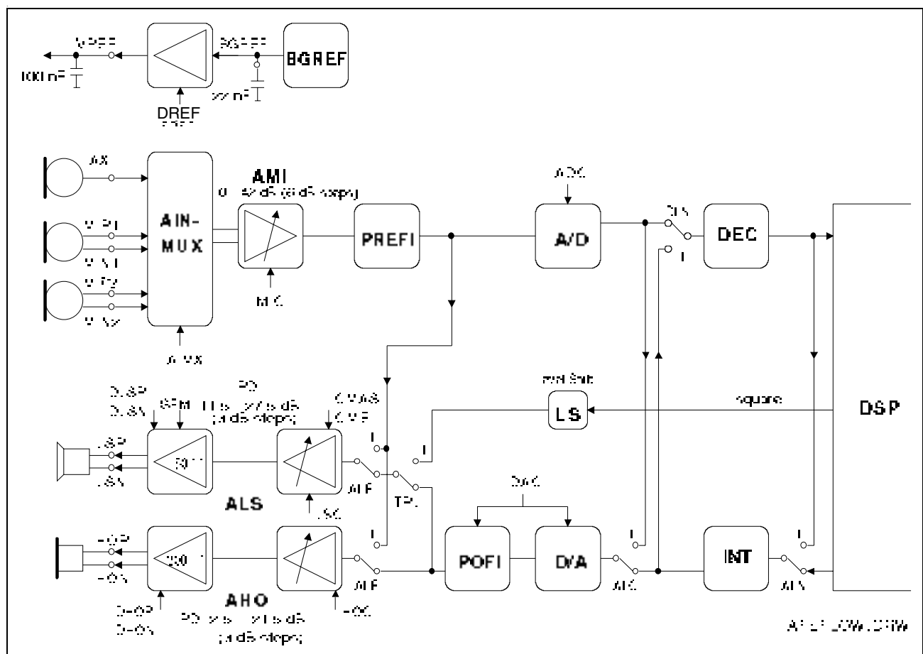
Figure 56 Block Diagram of AFE
