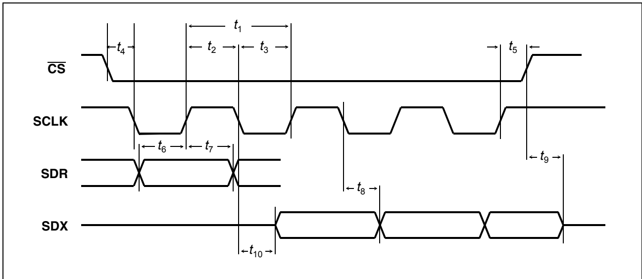
Figure 81 SCI Interface
