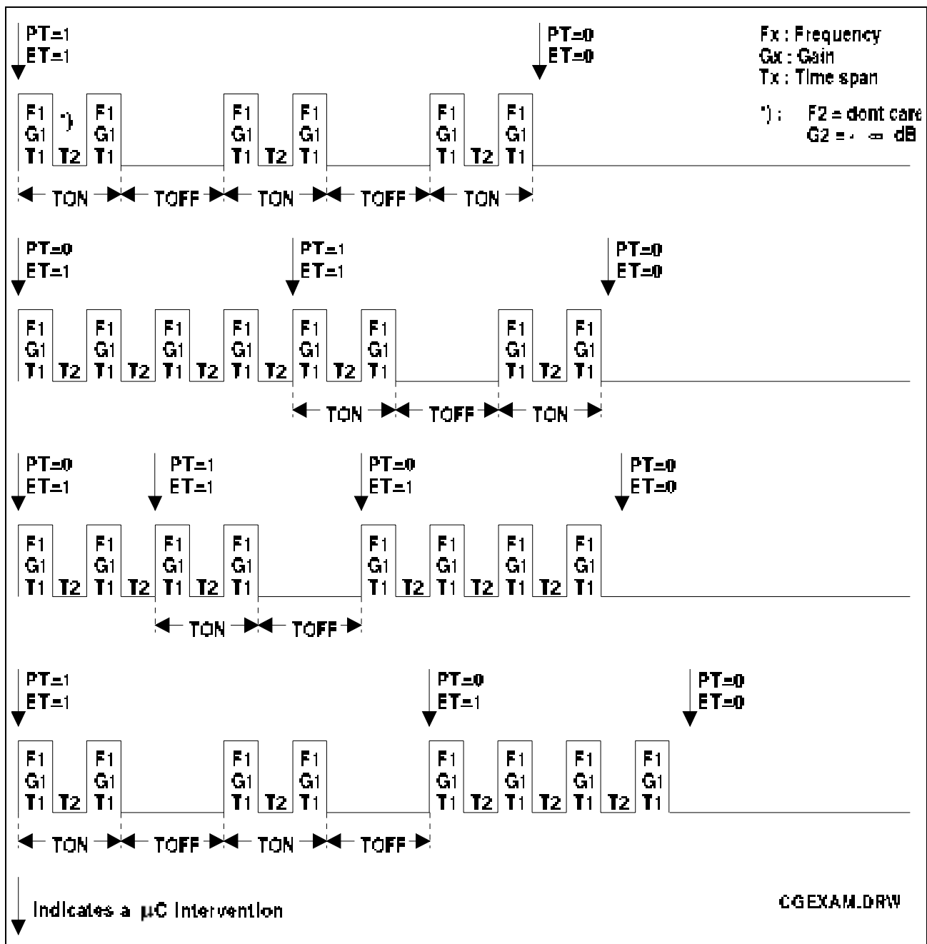
Figure 61 Typical Control Generator Applications
