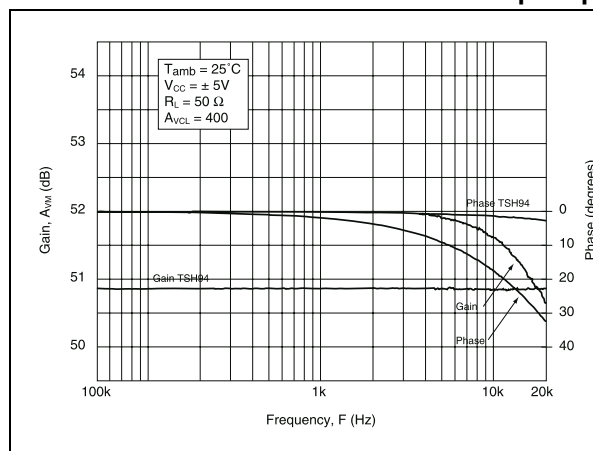
Figure 7. Audio bandwidth frequency response and phase shift (TSH94 vs standard 15 MHz audio op-amp)
