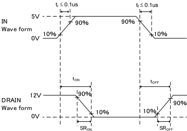
Figure 22. Switching Time
