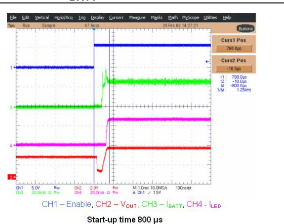
Figure 9. Start-up to torch mode 25 mA at V_{BATT} = 3.6V
