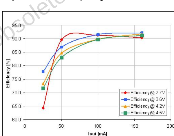
Figure 8. Efficiency vs I_O in torch mode
