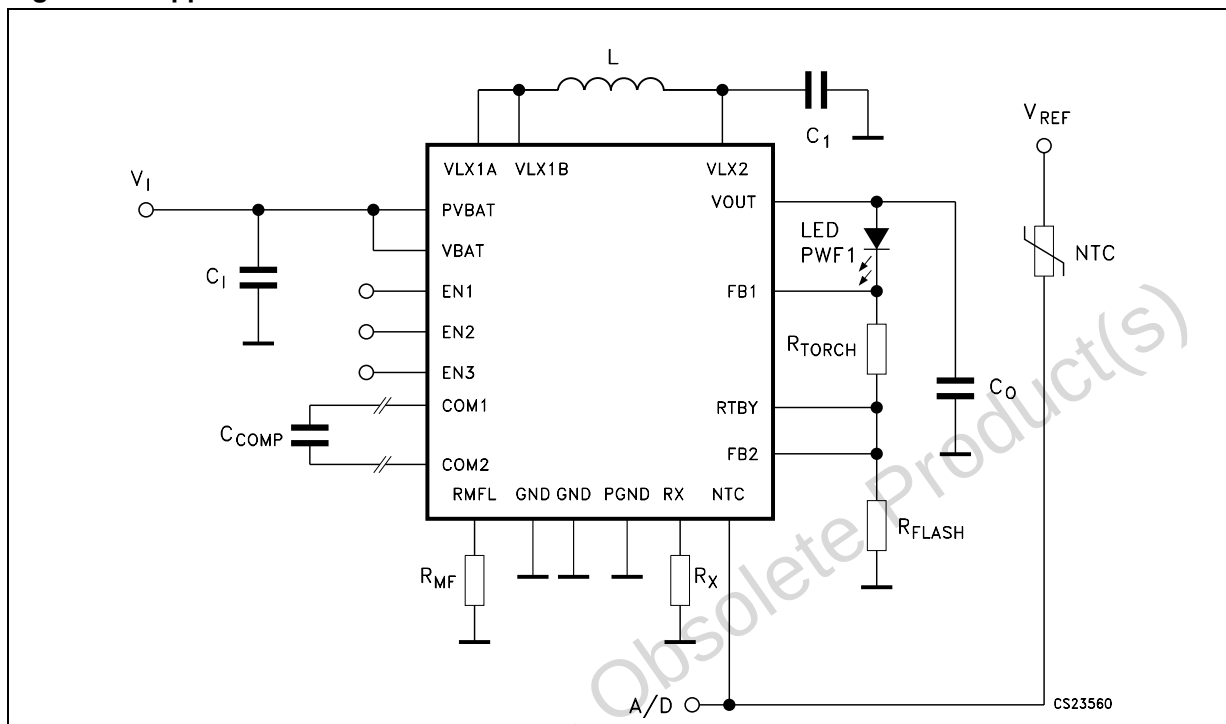
Figure 1. Application circuit
