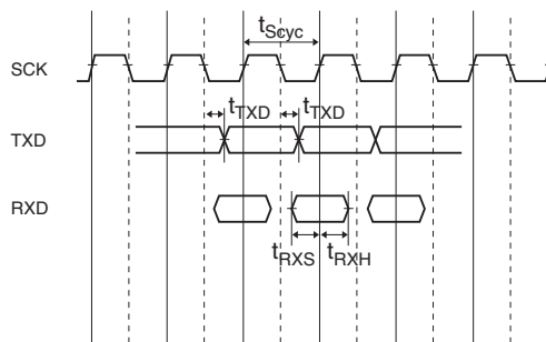
Figure 23.62 SCI I/O Synchronous Mode Clock Timing
