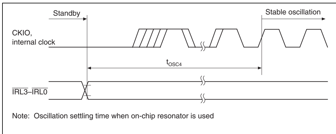
Figure 23.8 Standby Return Oscillation Settling Time (Return by \overline{\text{IRL3}}\text{--}\overline{\text{IRL0}} )
