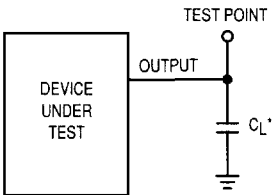
Figure 2. Test Circuit
