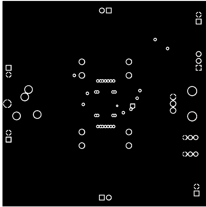
FIGURE 6. Bottom Layer
