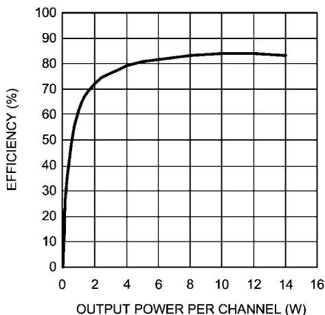
Efficiency vs Output Power V_{DD} = 15V, R_L = 8\Omega (both channels driven and measured)
