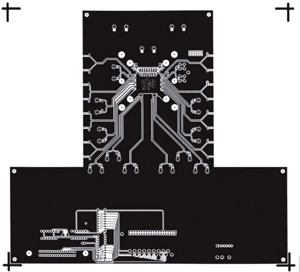
Figure 44. Circuit Side
