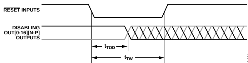
Figure 31. Asynchronous Reset
