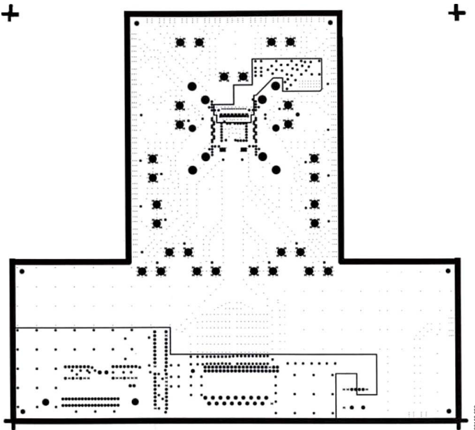
Figure 50. INT2 (V CC )
