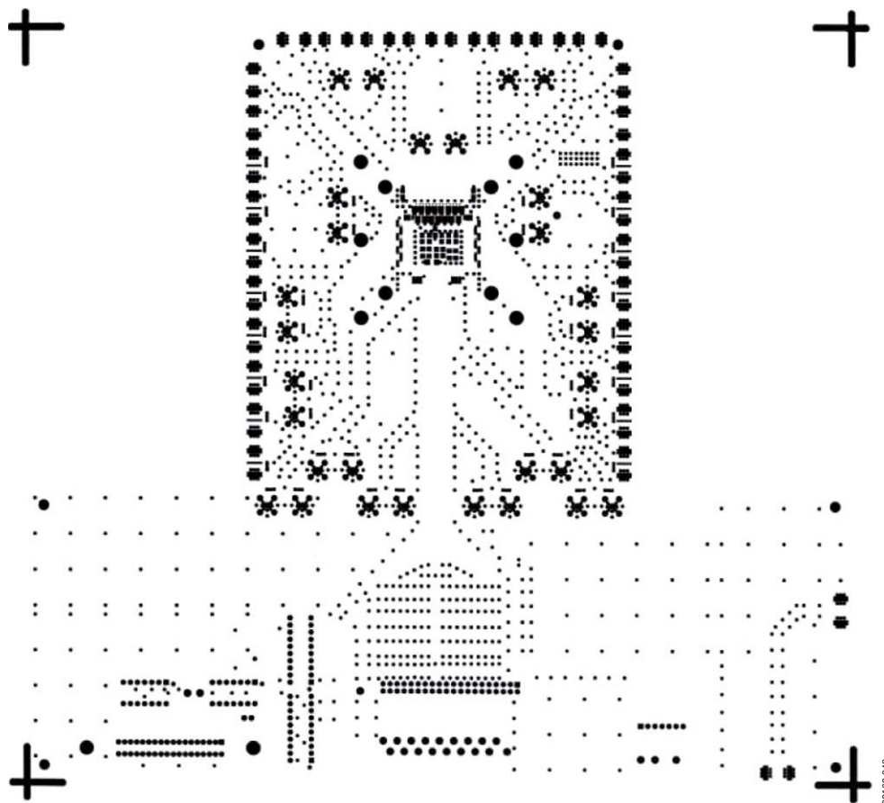
Figure 48. Solder Mask Bottom
