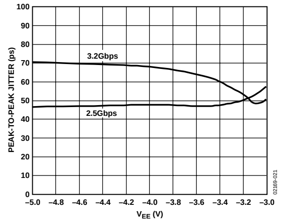
Figure 21. Jitter vs. Supply, PRBS 23
