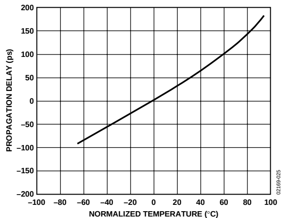
Figure 25. Propagation Delay, Normalized at 25°C vs. Temperature
