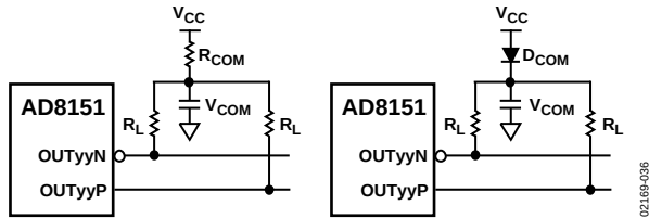
Figure 36. Output Pull-Up Networks for PECL/ECL: a) 100 k \Omega and b) 10 k \Omega
