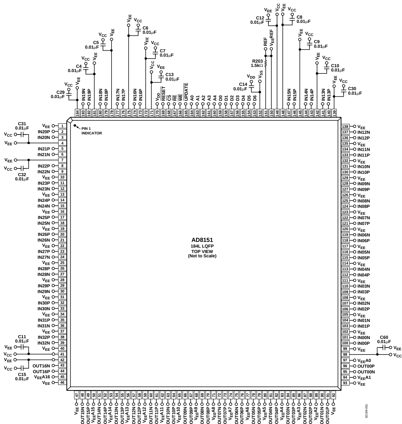
Figure 51. Bypassing Schematic
