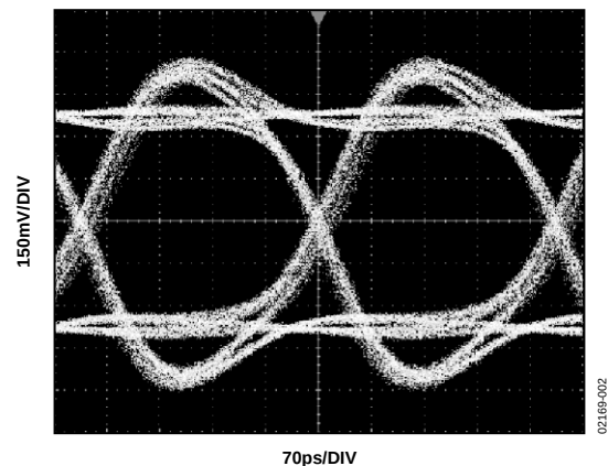
Figure 2. Eye Pattern, 3.2 Gbps, PRBS 23
