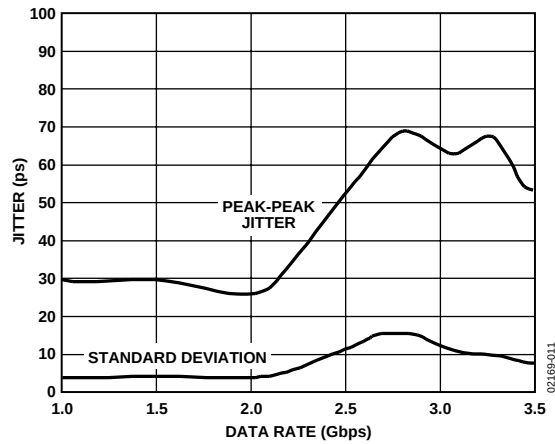
Figure 11. Jitter vs. Data Rate, PRBS 23
