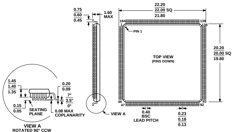
Figure S4. 184-Lead Low Profile Quad Flat Package [LQFP] (ST-184) Dimensions shown in millimeters
