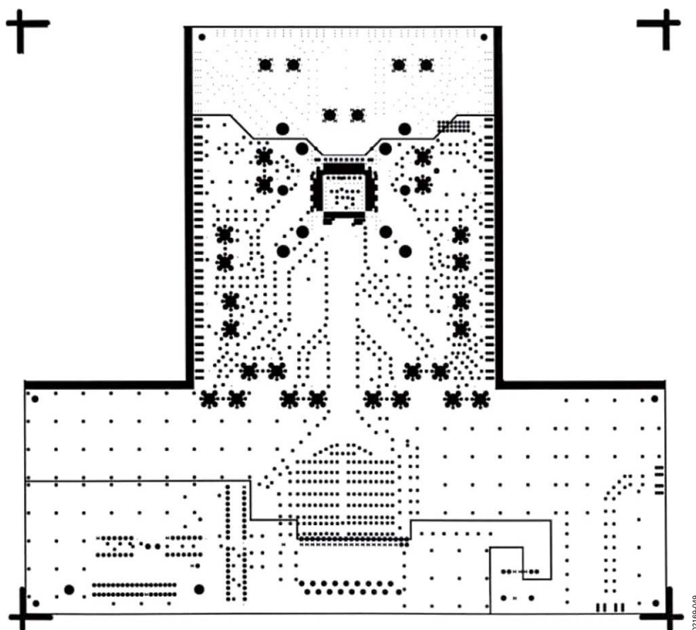
Figure 49. INT1 (V EE )
