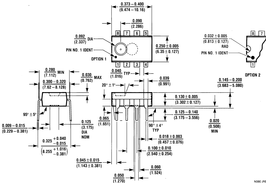
8-Lead (0.300" Wide) Molded Dual-In-Line Package Order Number LM4880N NS Package Number N08E
