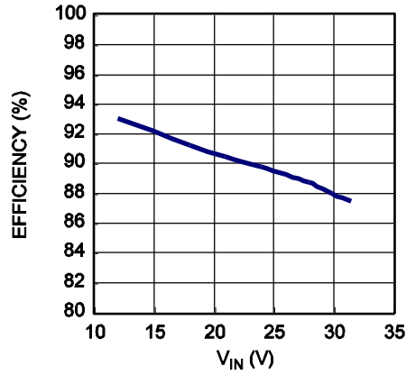
Efficiency Test
