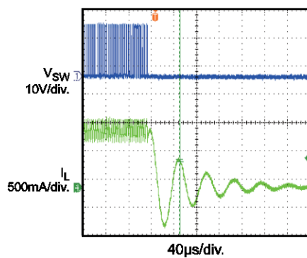
Open Protection
