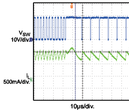
Short Protection
