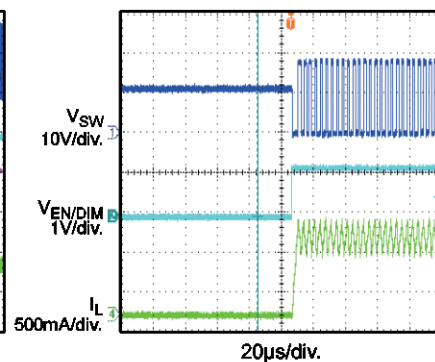
VEN Start-Up
