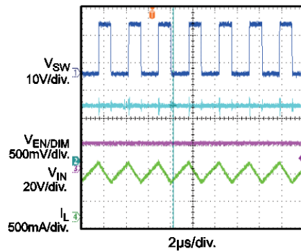
Analog Dimming
