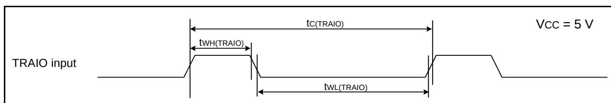
Figure 5.5 TRAIO Input Timing Diagram when V_{CC} = 5\text{ V}
