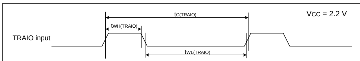
Figure 5.13 TRAIO Input Timing Diagram when V_{CC} = 2.2\text{ V}
