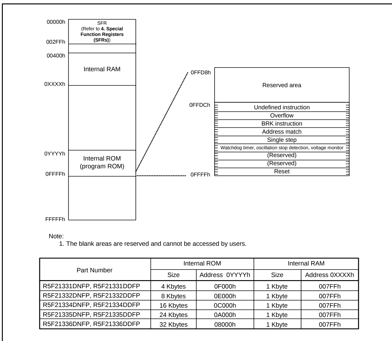
Figure 3.1 Memory Map of R8C/33D Group
