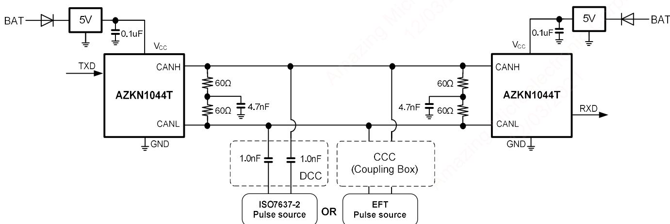
Figure 6. ISO 7637-2 DCC or EFT coupling test circuit for AZKN1044T.
