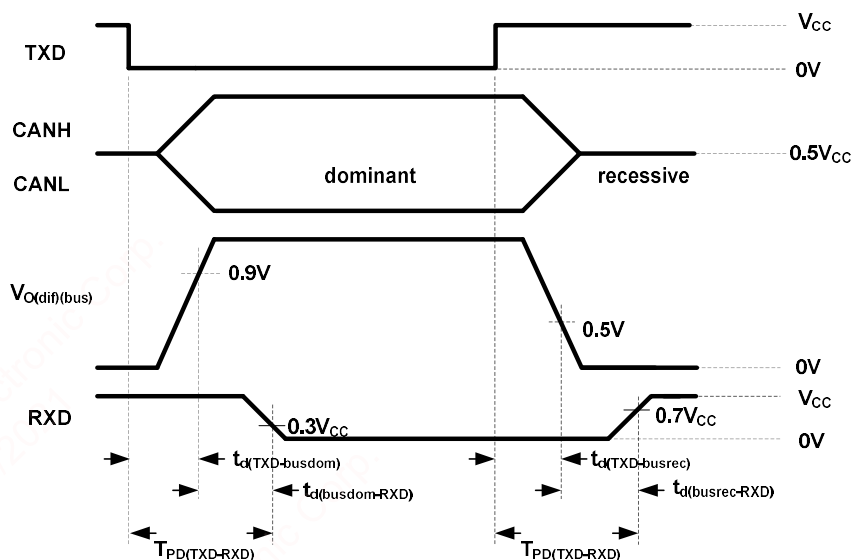
Figure 1. Timing diagram of the CAN transceiver.
