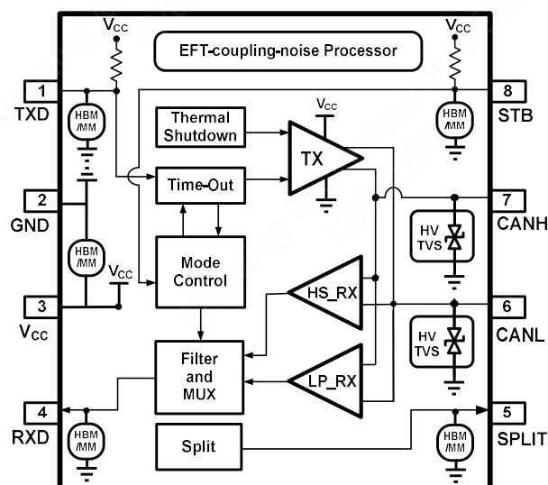
Functional Block of AZKN1044T
