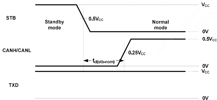
Figure 3. Timing diagram for the delay of the standby to normal mode.
