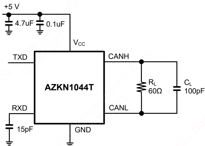
Figure 5. CAN transceiver timing test circuit.
