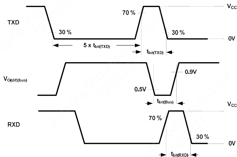
Figure 2. Timing diagram for loop delay symmetry.
