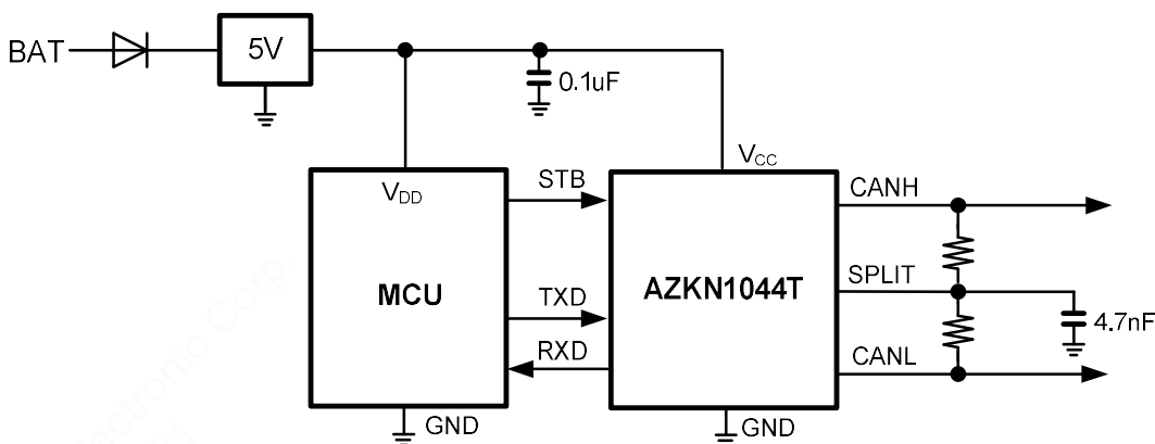
Figure 4. Typical application circuit for AZKN1044T with 5V MCU.
