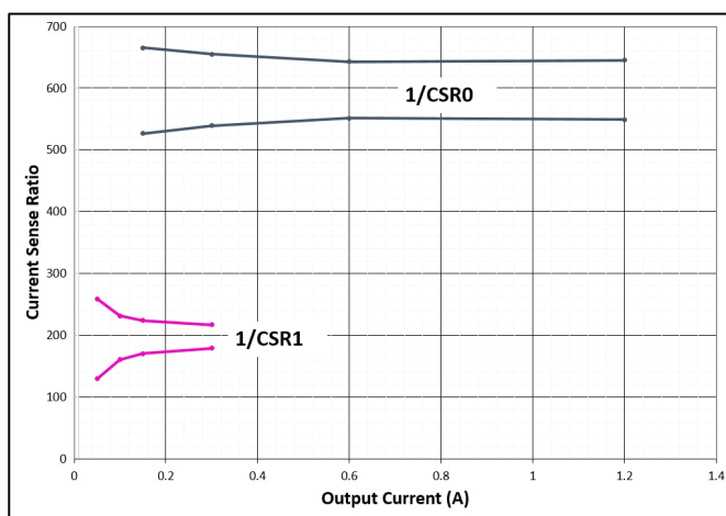
Figure 17. Current sensing ratio versus output current
