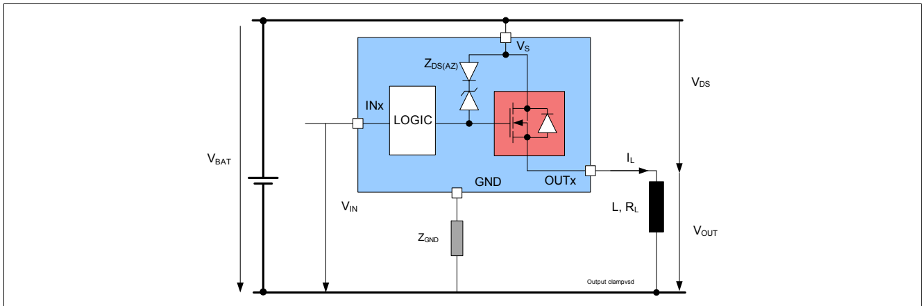
Figure 10 Output Clamp
