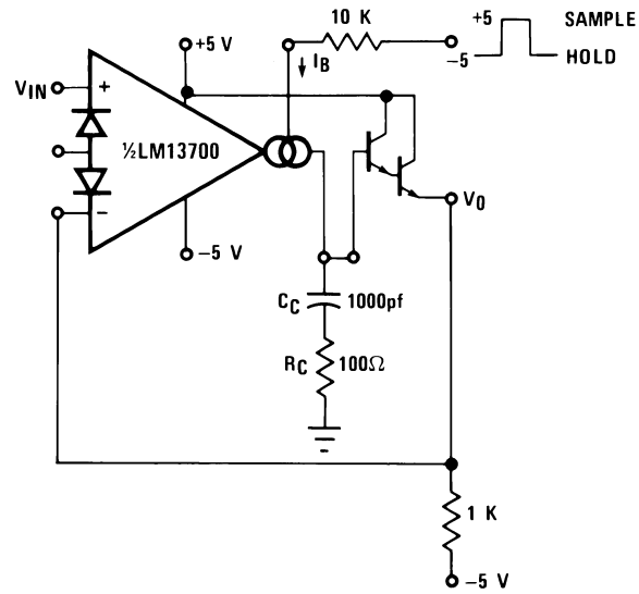
FIGURE 25. Sample-Hold Circuit
