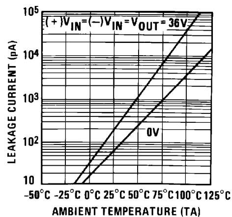
Leakage Current
