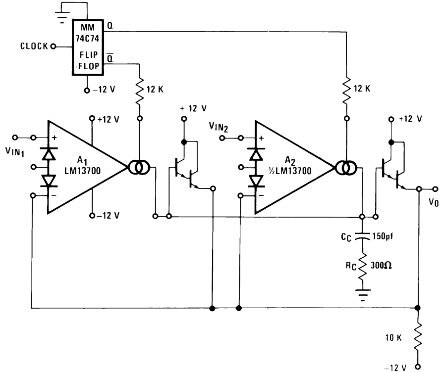
FIGURE 20. Multiplexer
