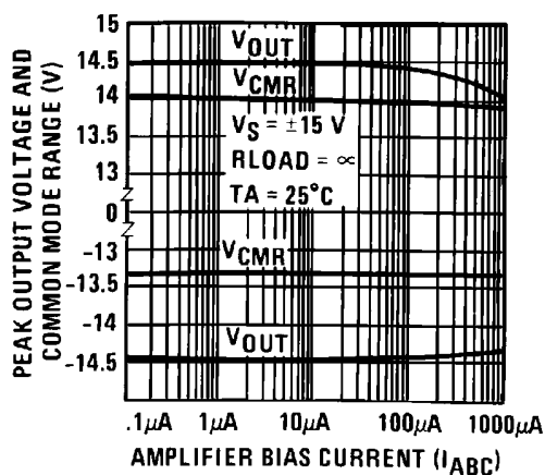
Peak Output Voltage and Common Mode Range
