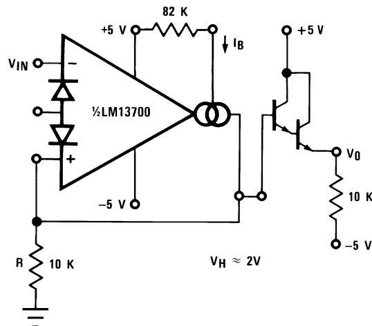
FIGURE 22. Schmitt Trigger
