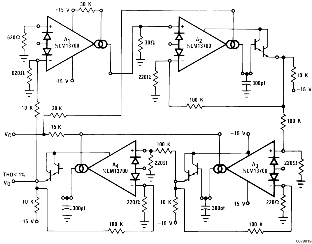
FIGURE 17. Sinusoidal VCO
