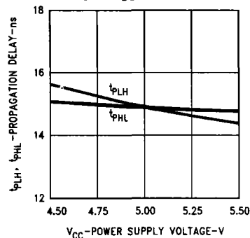
Receiver Propagation Delay vs V_{CC}
