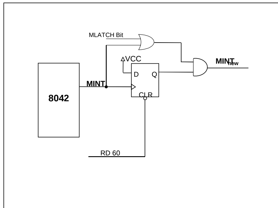
FIGURE 6 – MOUSE LATCH
