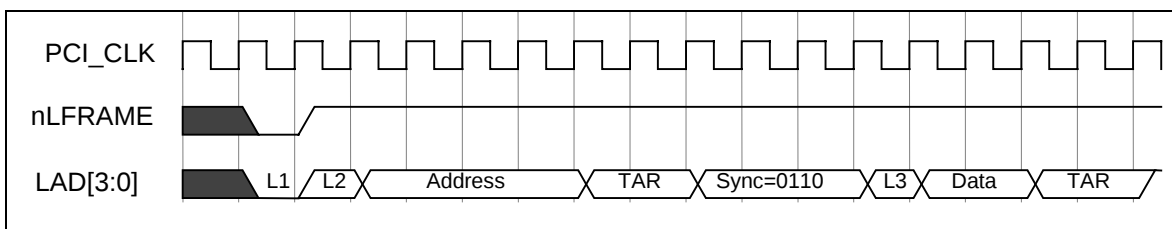
FIGURE 19 – I/O READ
