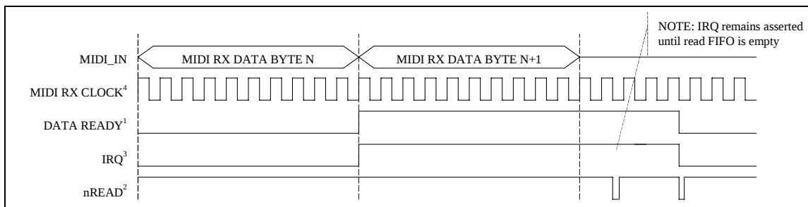
FIGURE 3 – MPU-401 INTERRUPT
