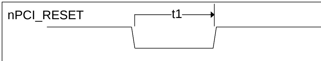
FIGURE 15 – RESET TIMING
