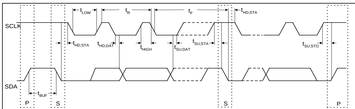
FIGURE 44 – SMBUS TIMING
