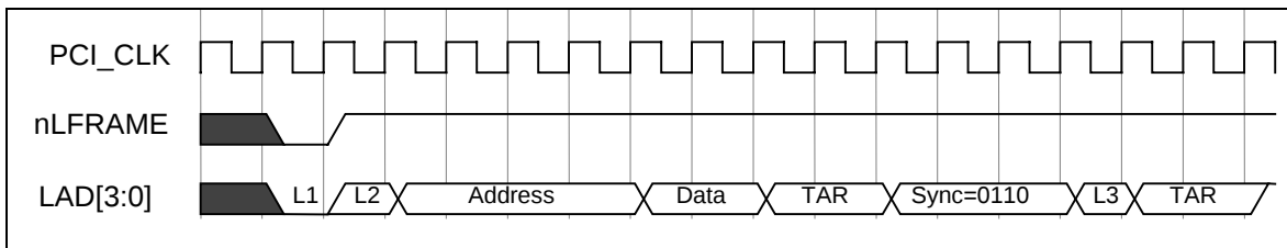
FIGURE 18 – I/O WRITE
