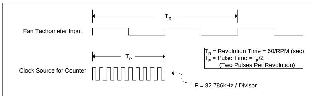
FIGURE 8 – FAN TACHOMETER INPUT AND CLOCK SOURCE
