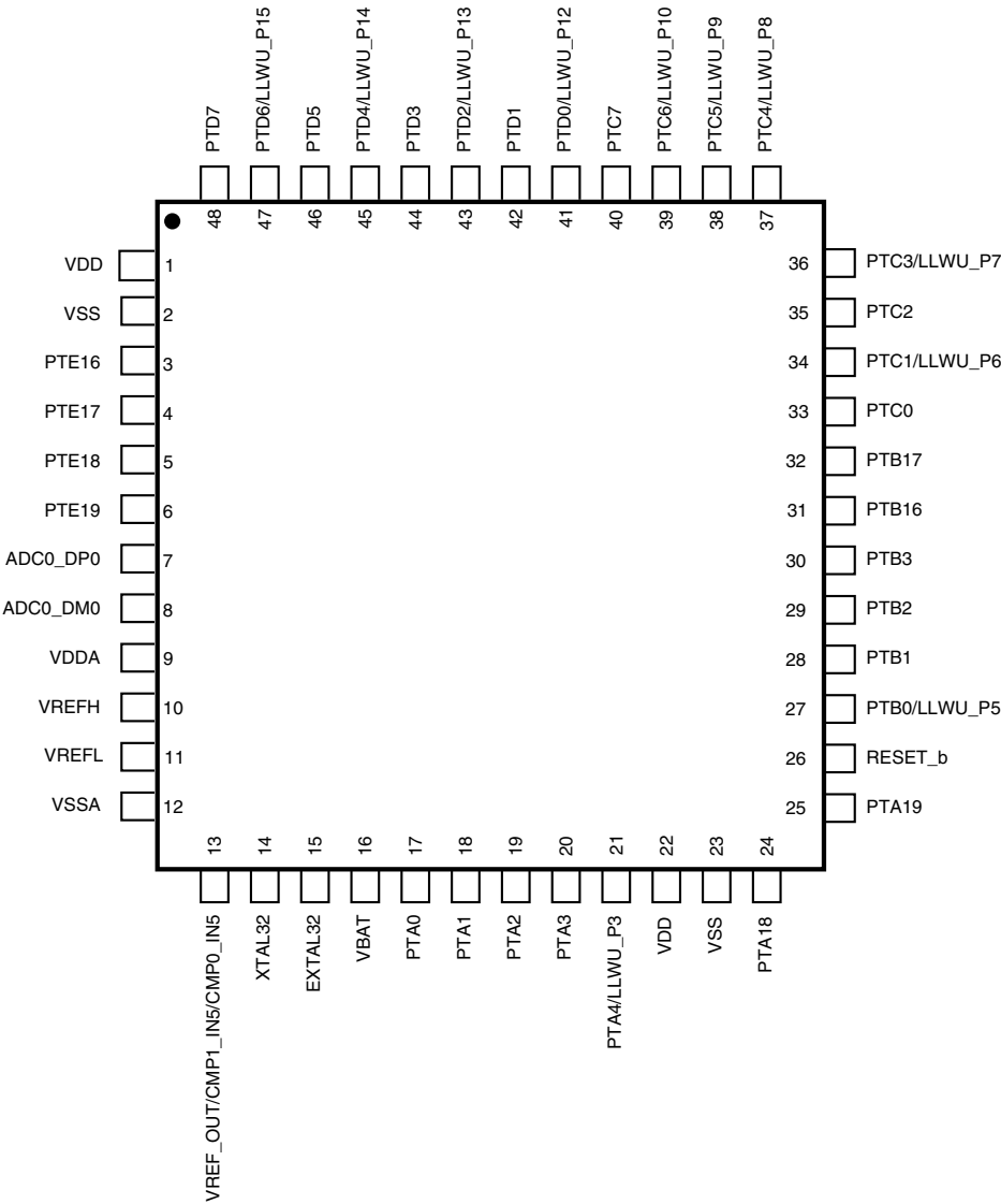
Figure 23. K10 48 LQFP/QFN Pinout Diagram
