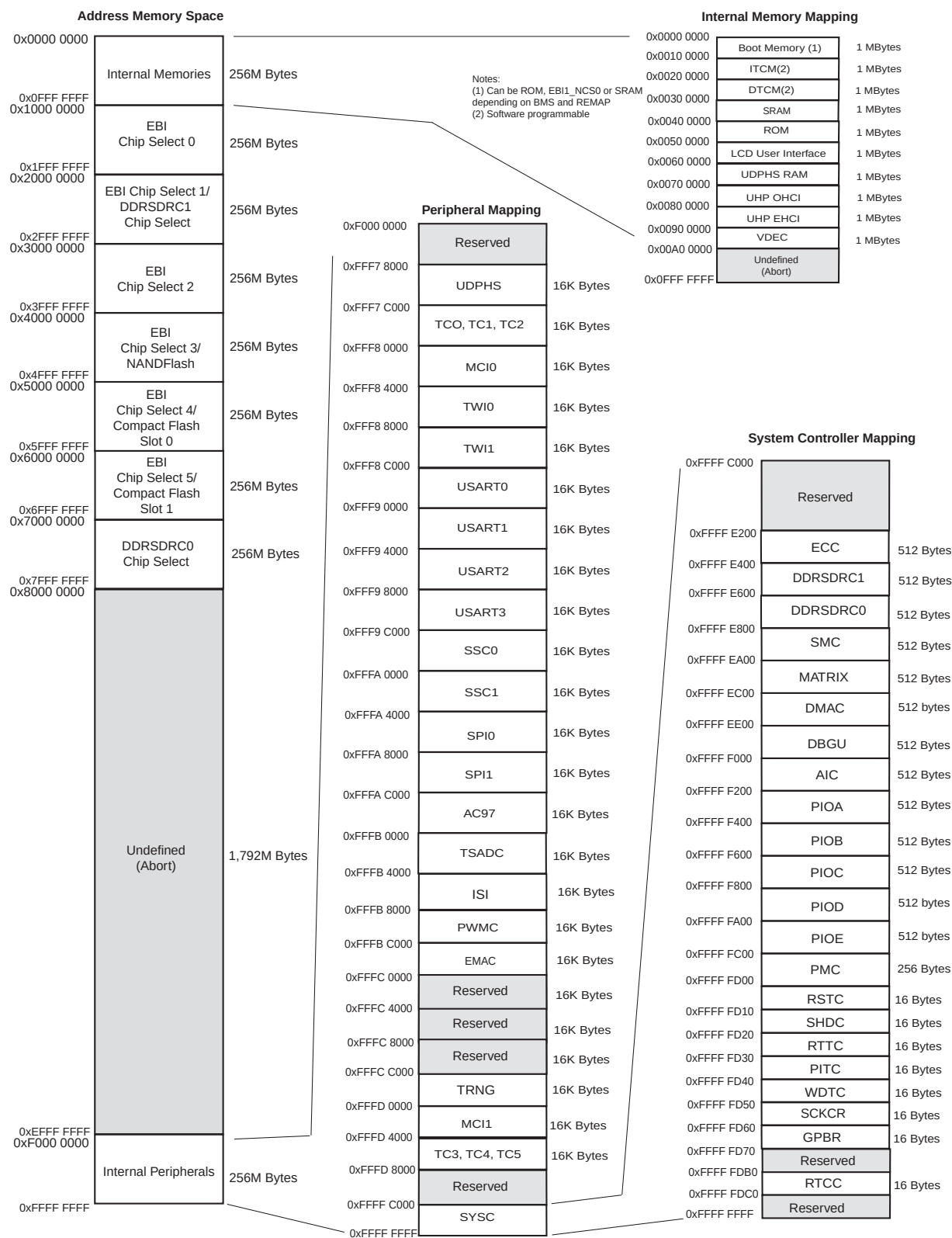
Figure 7-1. SAM9M10 Memory Mapping
