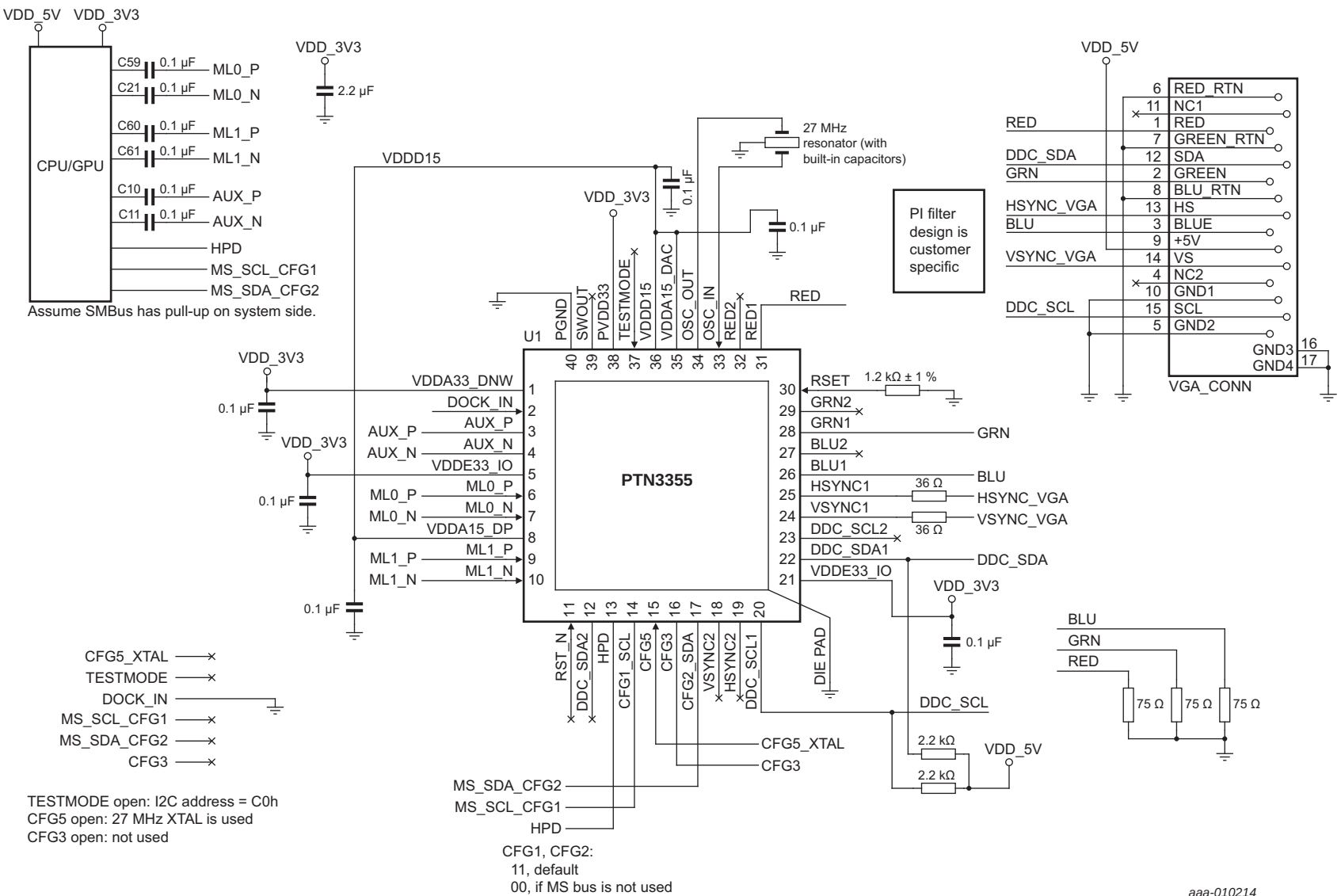
Fig 5. Application with LDO mode
