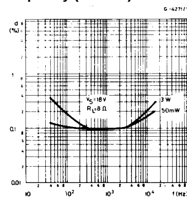
Figure 8. Distortion vs. frequency ( R_L = 8\Omega )
