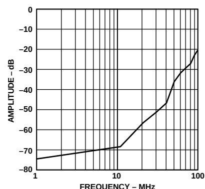
Figure 16. CMR vs. Input Frequency (Input Span = 2 V, V_{CM} = 2.5\text{ V} )
