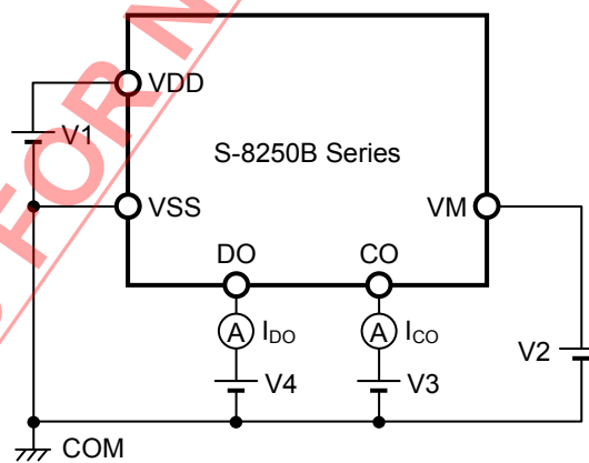
Figure 7 Test Circuit 4
