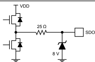
Figure 18h. SDO Output
