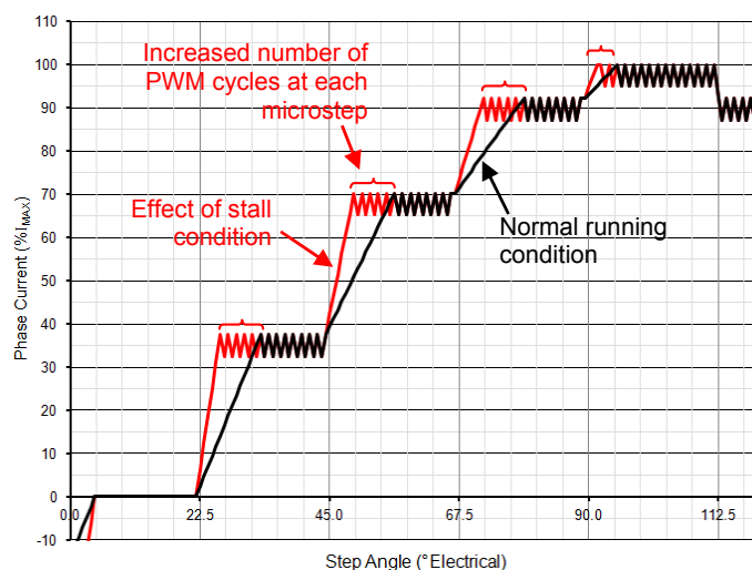
Figure 5: Effect of Stall Condition on Current Rise
