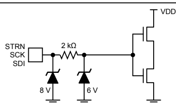
Figure 18e. STRN, SCK, SDI Inputs
