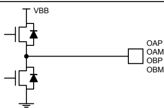
Figure 18i. Phase Outputs
