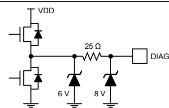
Figure 18j. DIAG Output
