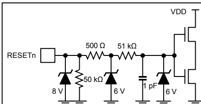
Figure 18g. RESETn Input
