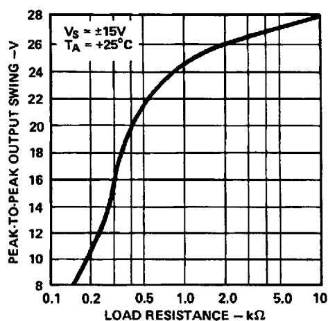
Figure 11. Output Voltage Swing vs. Load Resistance
