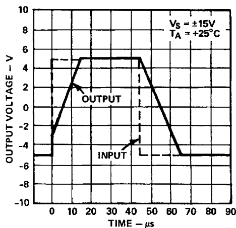
Figure 9. Voltage Follower Large Signal Pulse Response
