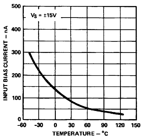
Figure 1. Input Bias Current vs. Temperature
