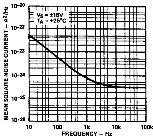
Figure 8. Input Noise Current vs. Frequency
