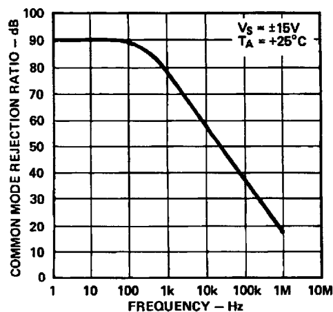
Figure 5. Common-Mode Rejection vs. Frequency
