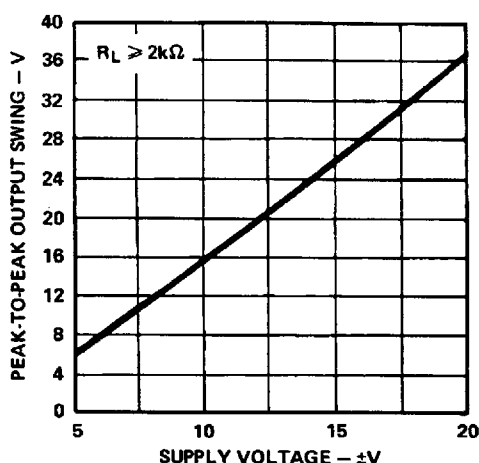
Figure 10. Output Voltage Swing vs. Supply Voltage
