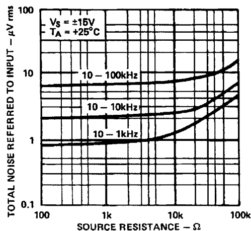
Figure 6. Broad Band Noise vs. Source Resistance
