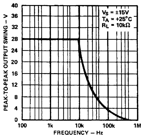
Figure 12. Output Voltage Swing vs. Frequency
