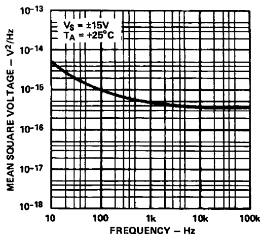
Figure 7. Input Noise Voltage vs. Frequency
