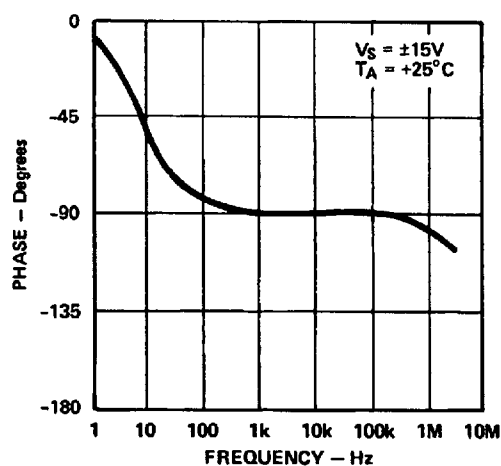
Figure 4. Open-Loop Phase Response vs. Frequency
