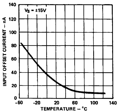
Figure 2. Input Offset Current vs. Temperature
