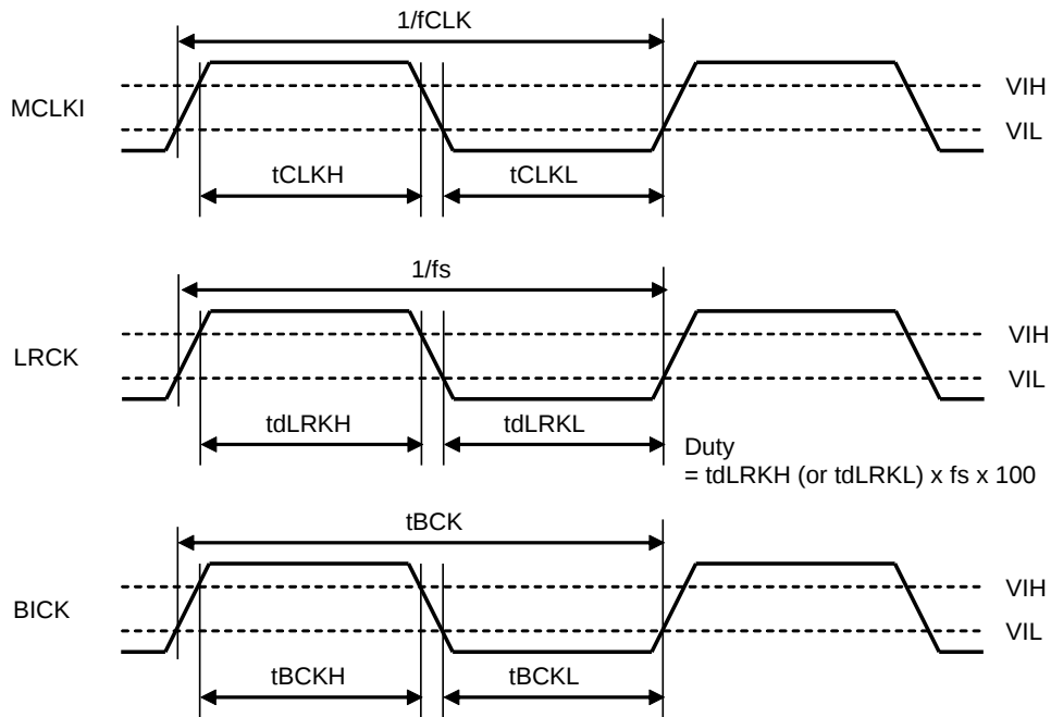
Figure 2. Clock Timing (TDM1/0 bits = "00" & Slave mode)
