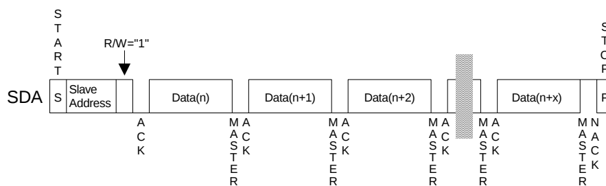
Figure 37. CURRENT ADDRESS READ
