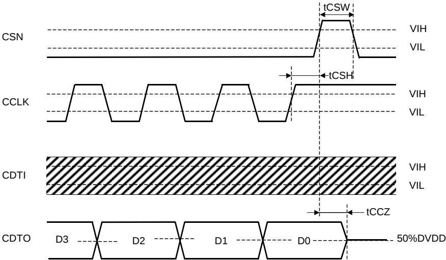
Figure 13. READ data output timing 2 (4-wire serial mode)
