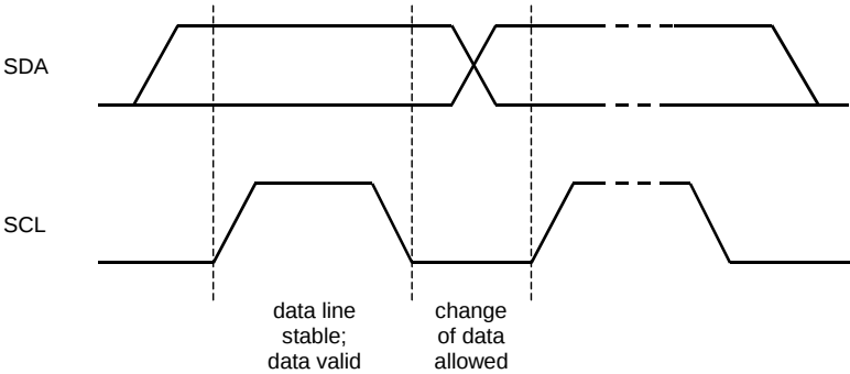
Figure 41. Bit Transfer on the I 2 C-Bus
