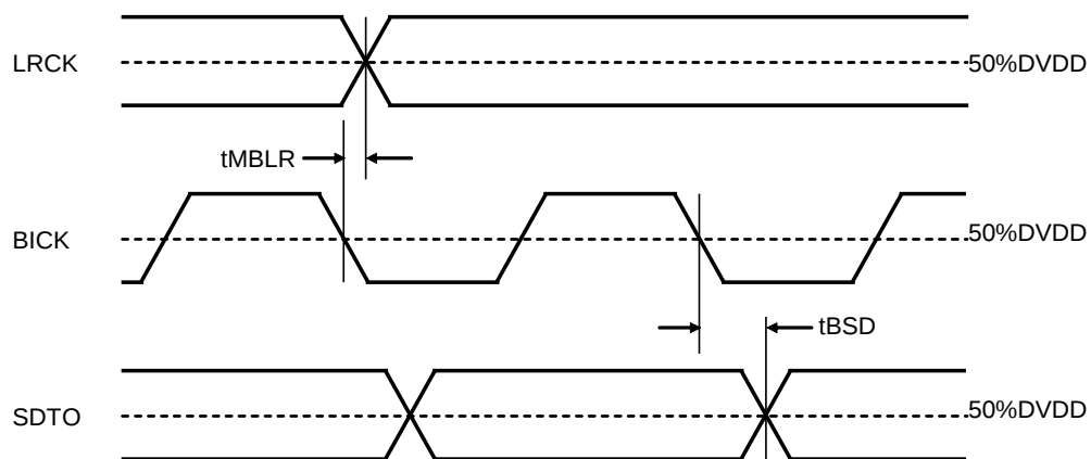
Figure 8. Audio Interface Timing (TDM1/0 bits = "00" &amp; Master mode)
