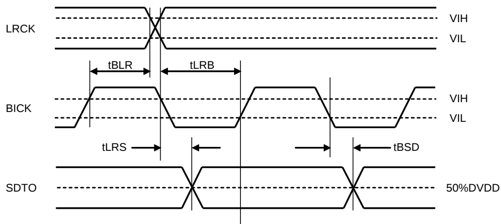
Figure 6. Audio Interface Timing (TDM1/0 bits = "00" &amp; Slave mode)
