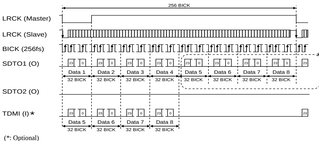
Figure 17. Mode1 Timing (TDM256 Mode (I 2 S))
