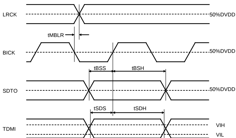
Figure 9. Audio Interface Timing (Except TDM1/0 bits = "00" &amp; Master mode)
