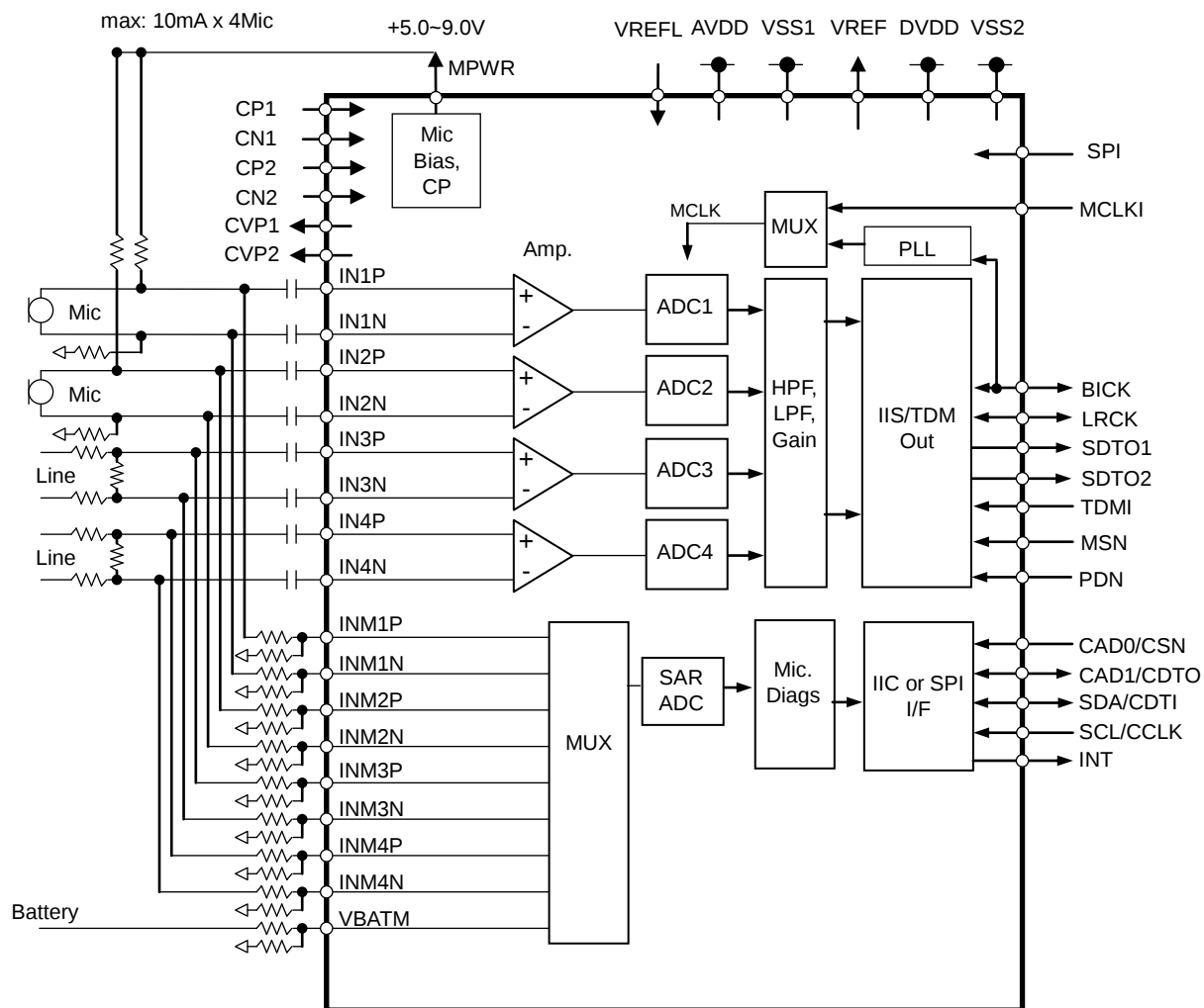
Figure 1. Block Diagram
