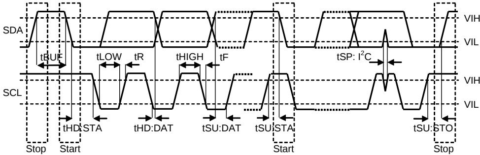
Figure 14. I²C Bus Timing
