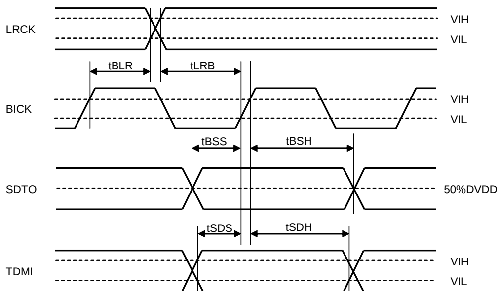
Figure 7. Audio Interface Timing (Except TDM1/0 bits = "00" &amp; Slave mode)
