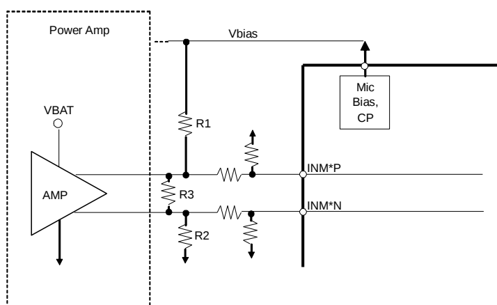
Figure 27. Booster Input Mode (INM*P/N pins)
