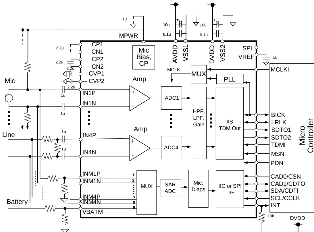
Figure 42. Typical Connection Diagram
