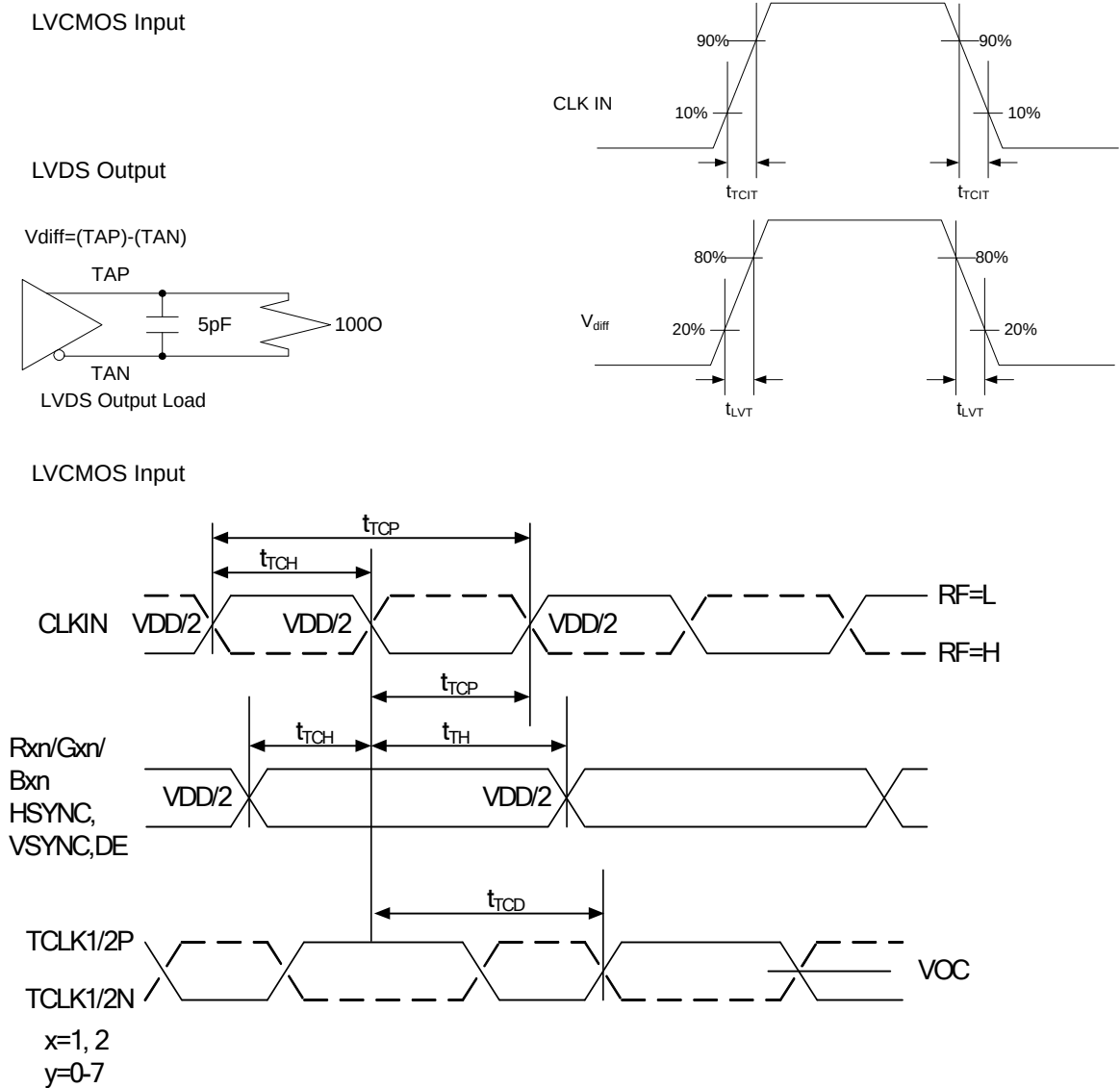
Fig.6 AC Timing Diagrams
