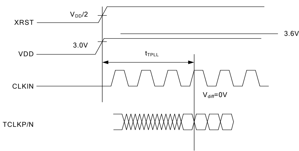
Fig.8 Phase Lock Loop Set Time
