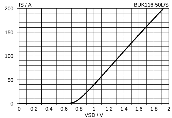
Fig.25. Typical reverse diode current, T_J = 25 \text{ °C} . I_S = f(V_{DS}) ; conditions: V_{IS} = 0 \text{ V} ; t_p = 250 \text{ μs}
