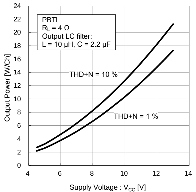
Figure 12. Output Power vs Supply Voltage (PBTL, R_L = 4\ \Omega )
