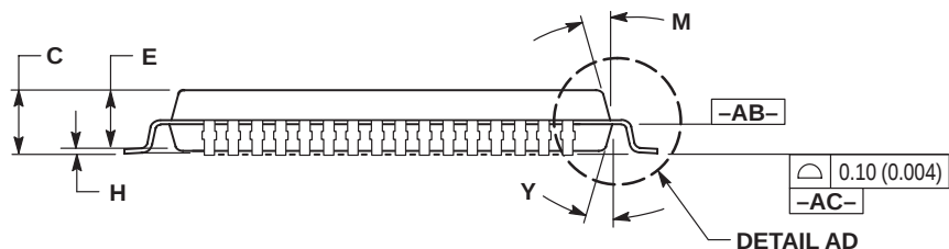
DETAIL AD
