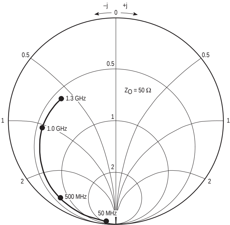
Figure 2. Typical HF Input Impedance
