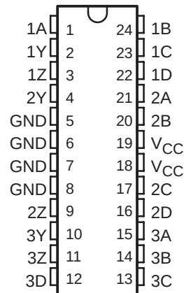
DW PACKAGE (TOP VIEW)
