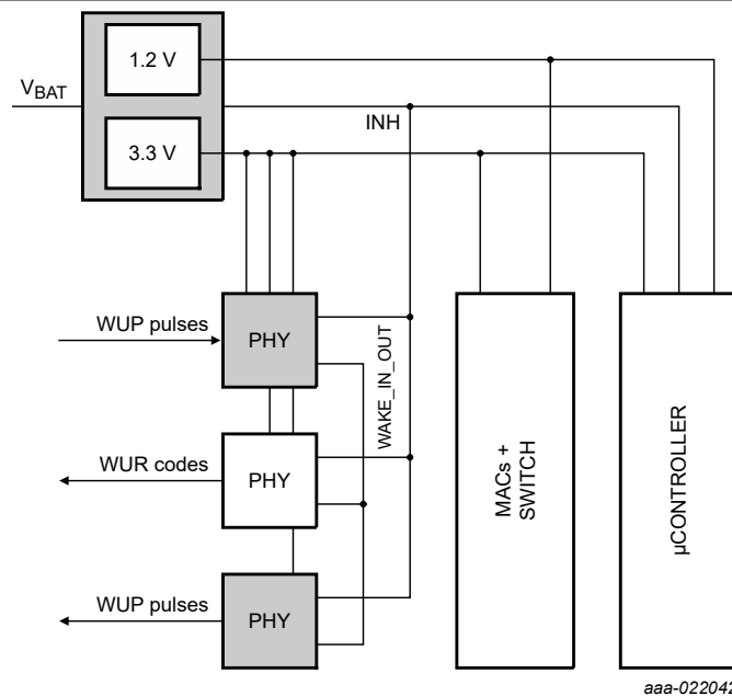
Figure 8. Wake-up request forwarding
