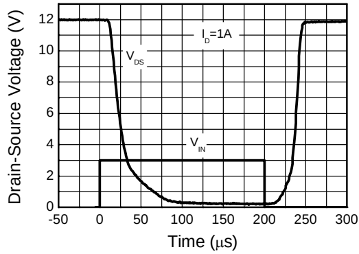
Switching Speed
