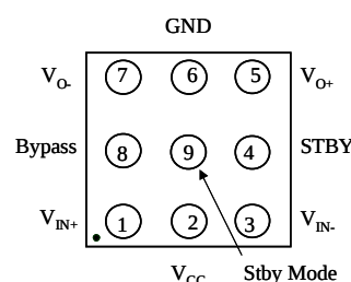
TS4994IQT - DFN10
