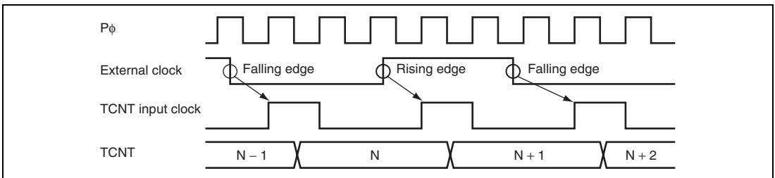
Figure 9.31 Count Timing in External Clock Operation
