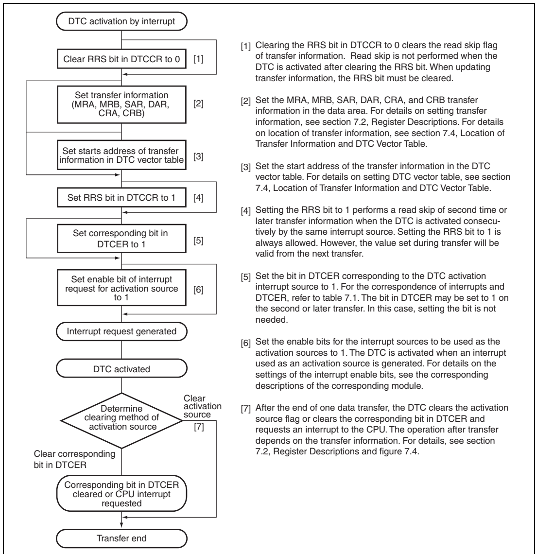
Figure 7.15 DTC with Interrupt Activation
