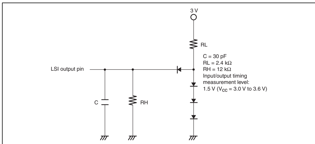
Figure 20.1 Output Load Circuit
