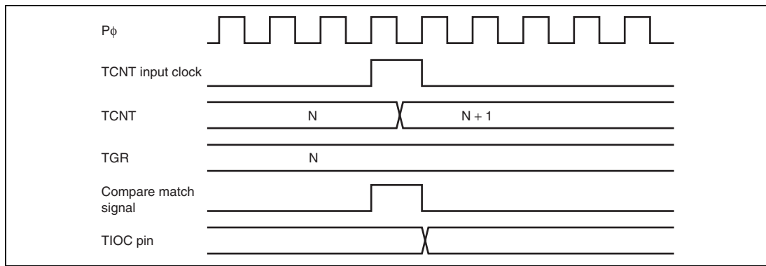
Figure 9.32 Output Compare Output Timing
