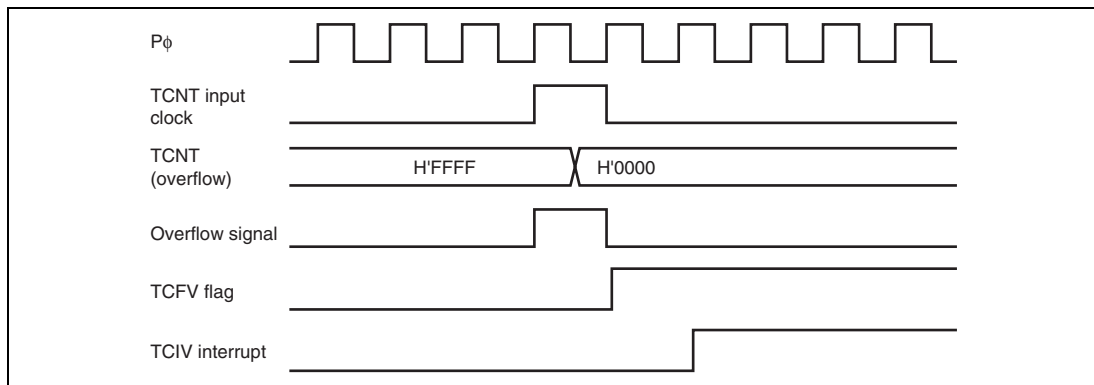
Figure 9.40 TCIV Interrupt Setting Timing
