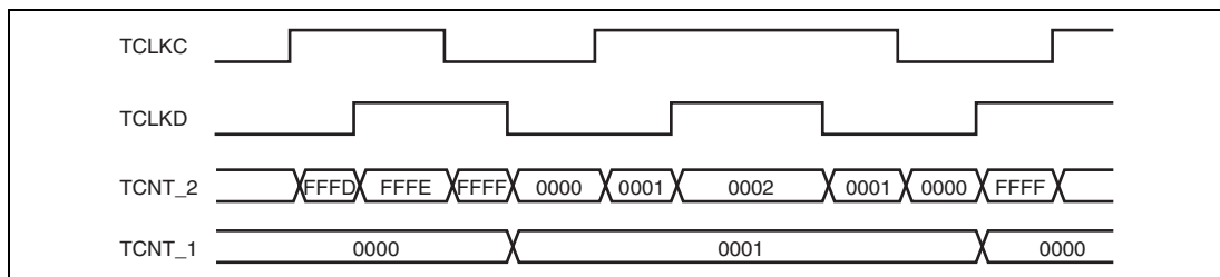
Figure 9.19 Example of Cascaded Operation (2)
