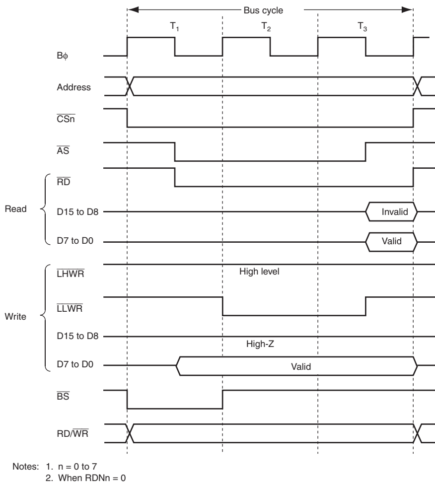
Figure 6.18 16-Bit 3-State Access Space Bus Timing (Word Access for Odd Address)
