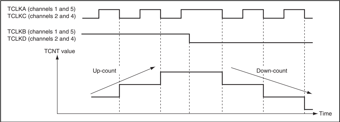
Figure 9.26 Example of Phase Counting Mode 2 Operation
