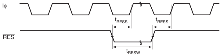
Figure 20.6 Reset Input Timing
