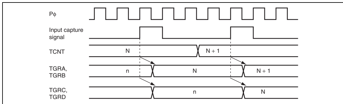
Figure 9.37 Buffer Operation Timing (Input Capture)
