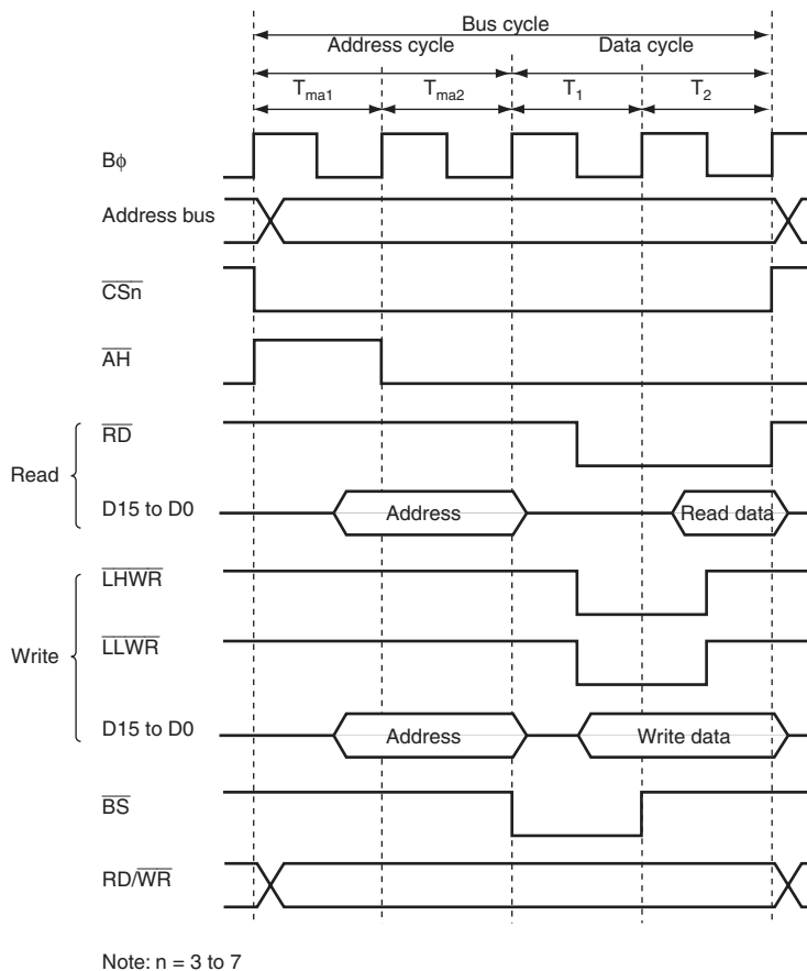
Figure 6.29 16-Bit Access Space Access Timing (ABWHn = 0, ABWLn = 1)
