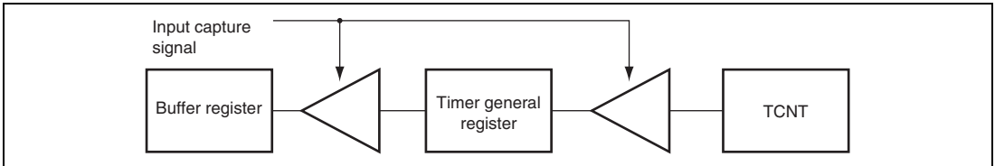
Figure 9.13 Input Capture Buffer Operation
