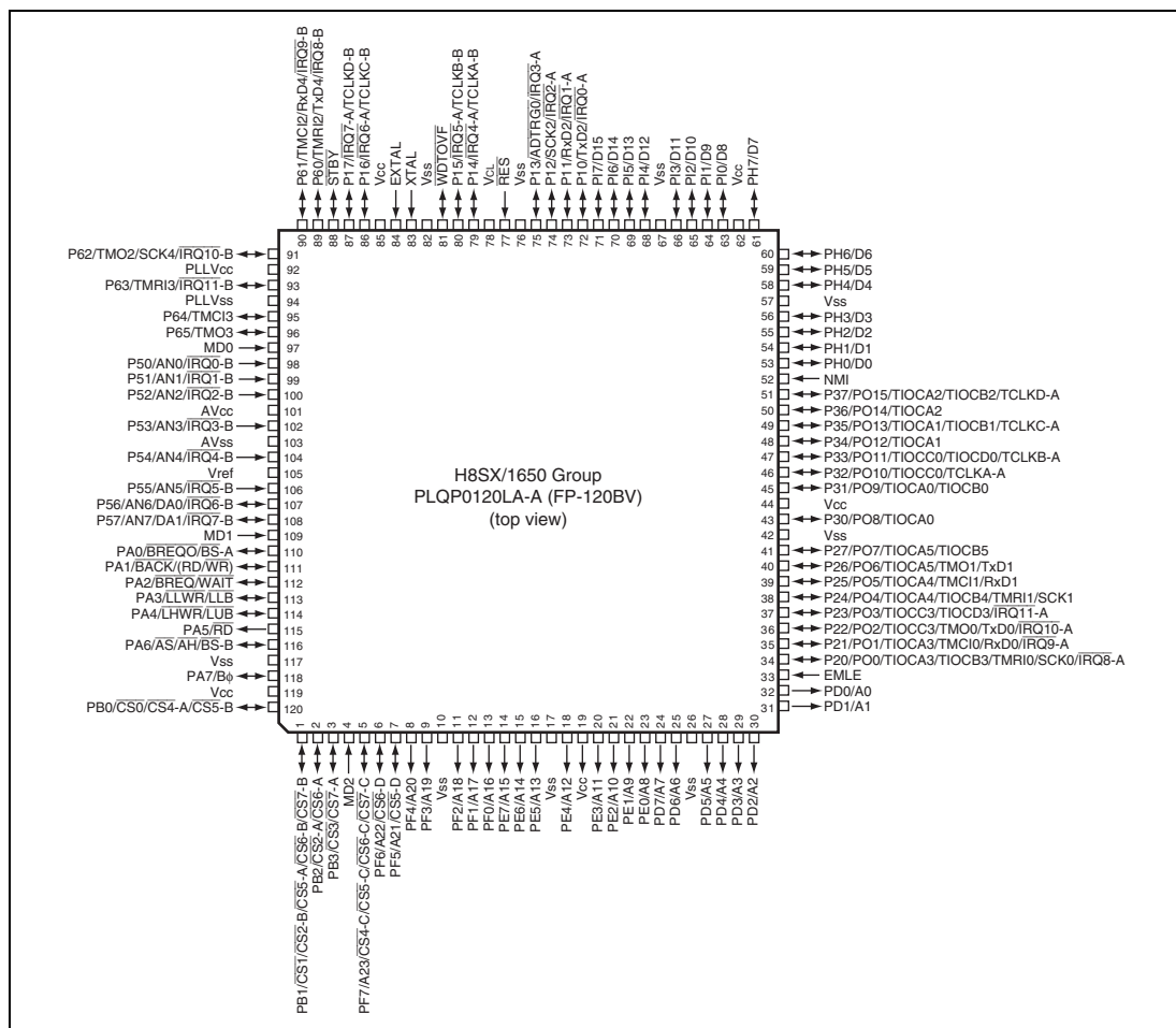
Figure 1.3 Pin Assignments
