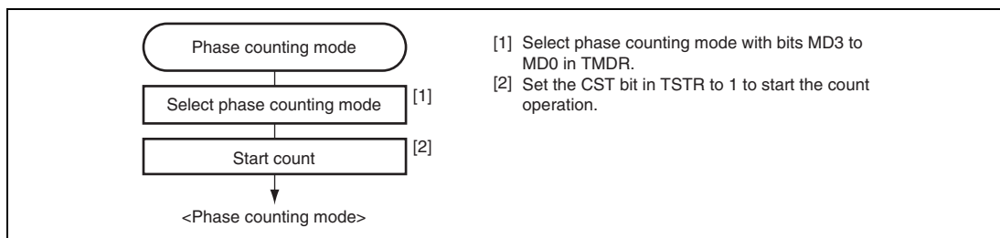
Figure 9.24 Example of Phase Counting Mode Setting Procedure
