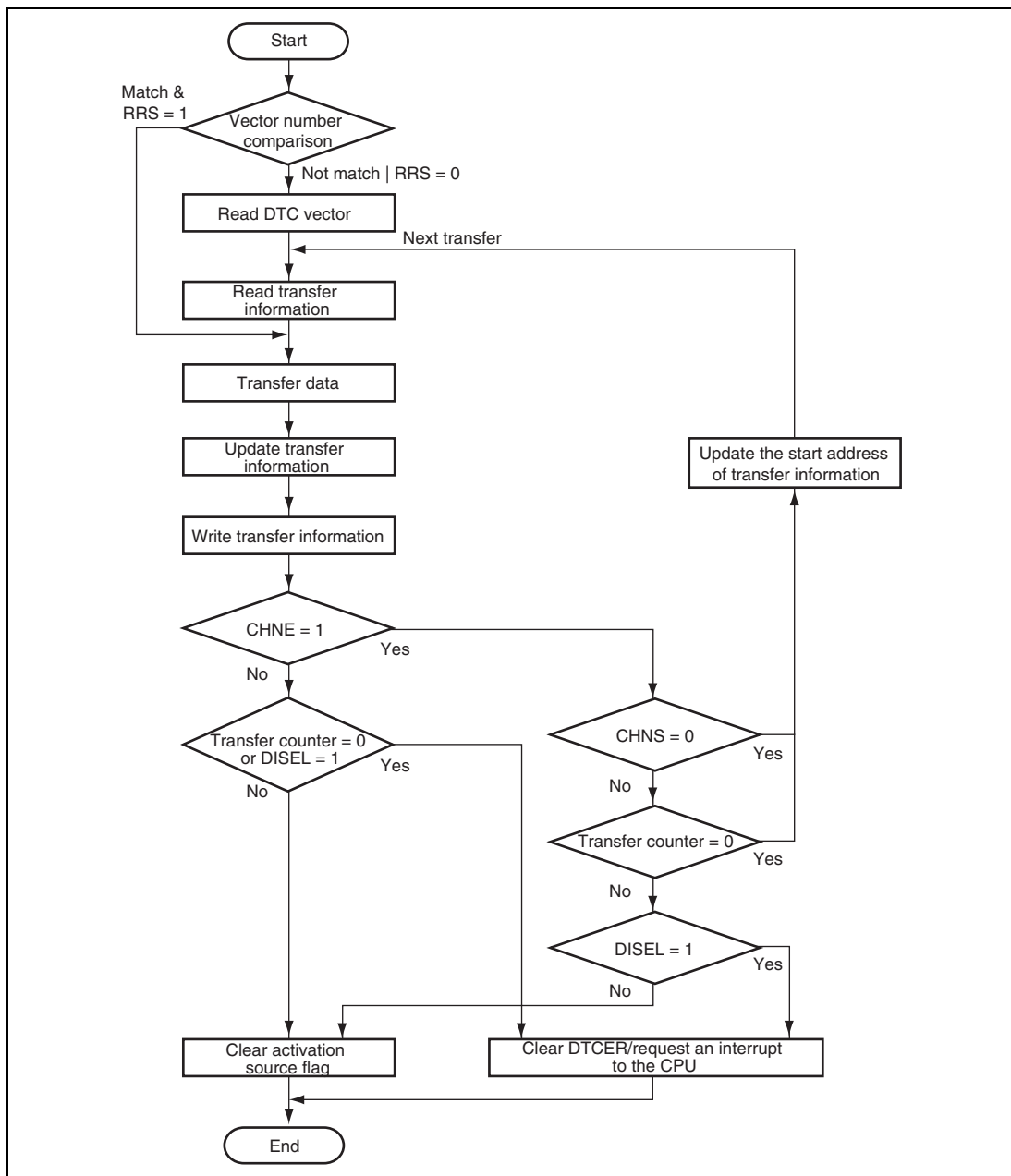
Figure 7.4 Flowchart of DTC Operation
