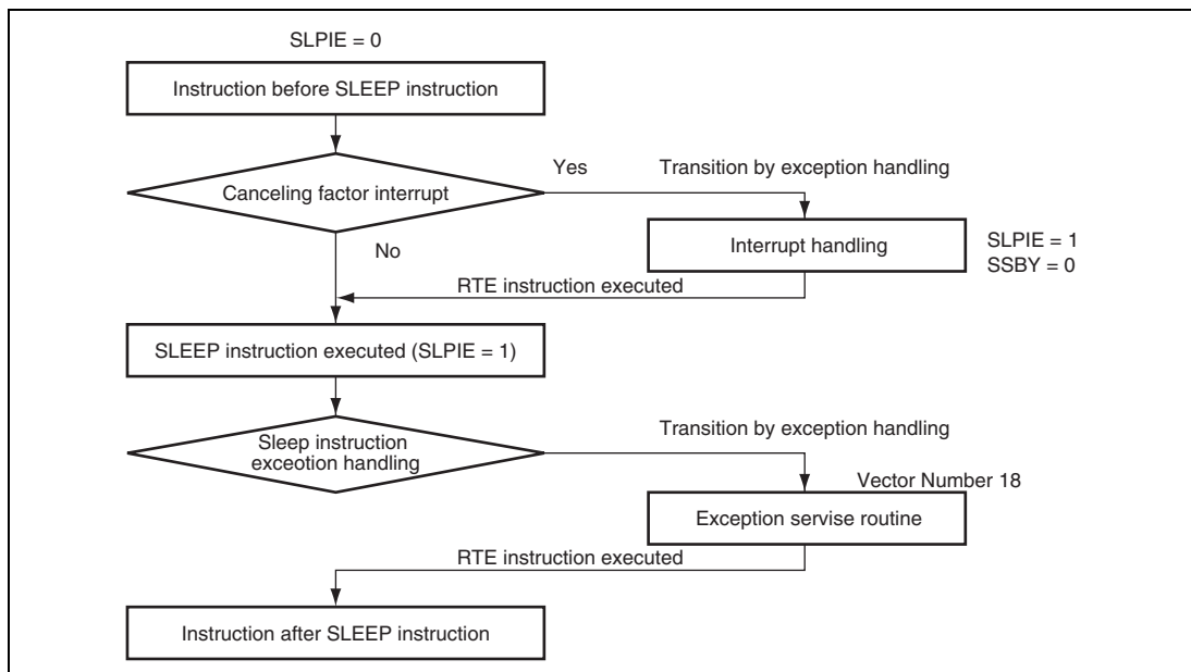
Figure 18.7 When Canceling Factor Interrupt is Generated before SLEEP Instruction Execution (Sleep Instruction Exception Handling Initiated)
