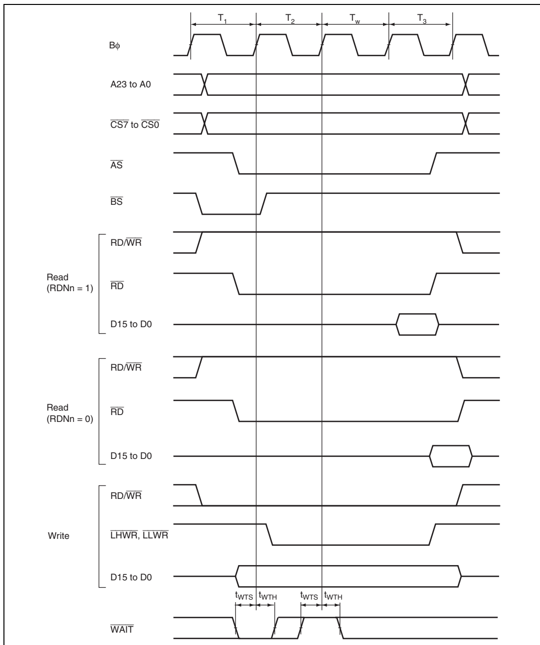
Figure 20.10 Basic Bus Timing: Three-State Access, One Wait
