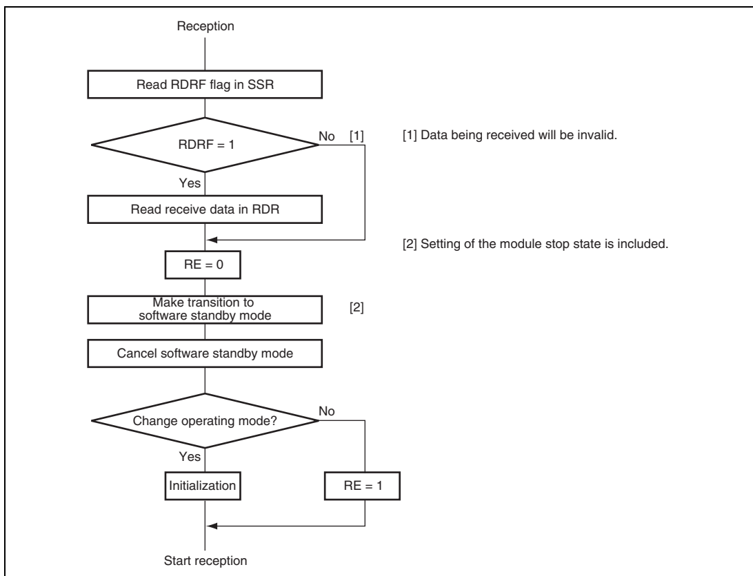
Figure 13.37 Sample Flowchart for Transition to Software Standby Mode during Reception
