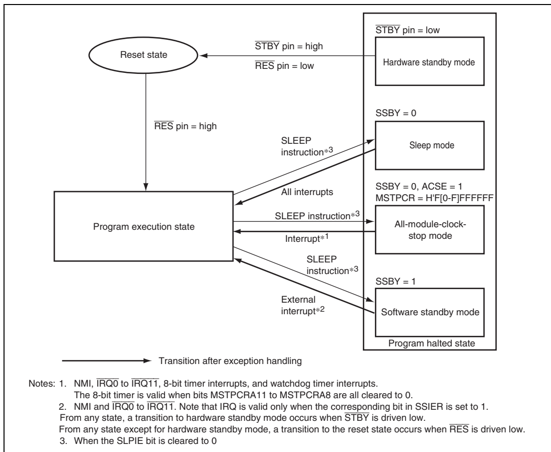
Figure 18.1 Mode Transitions
