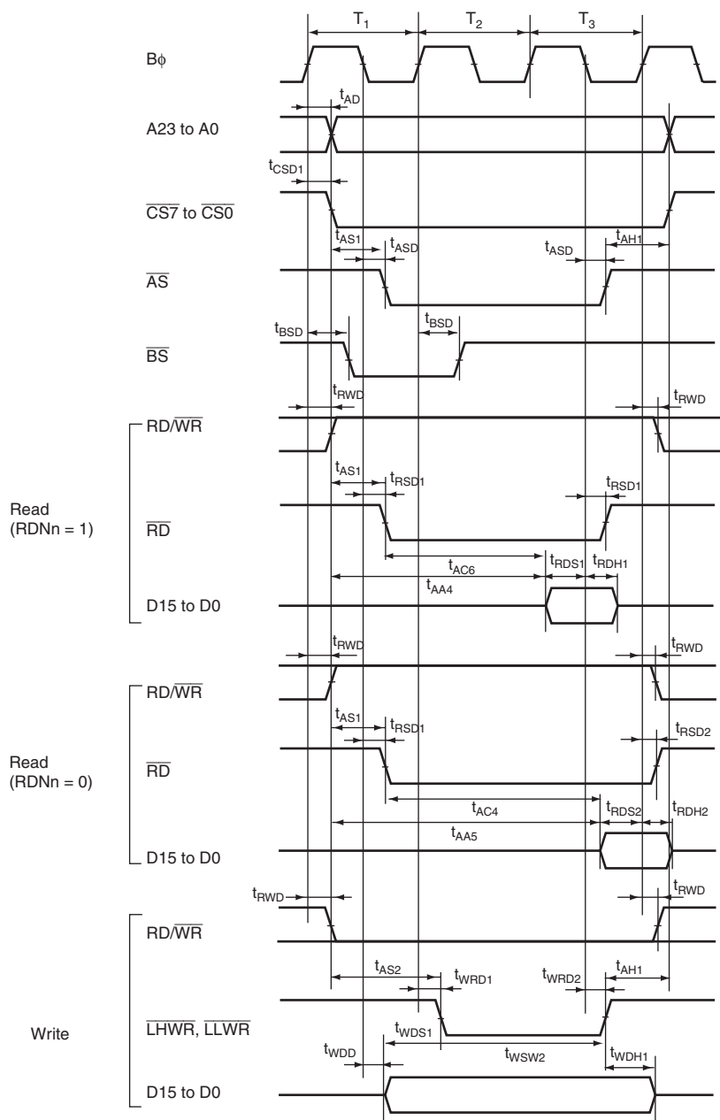
Figure 20.9 Basic Bus Timing: 3-State Access
