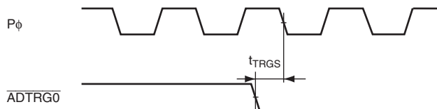
Figure 20.31 A/D Converter External Trigger Input Timing
