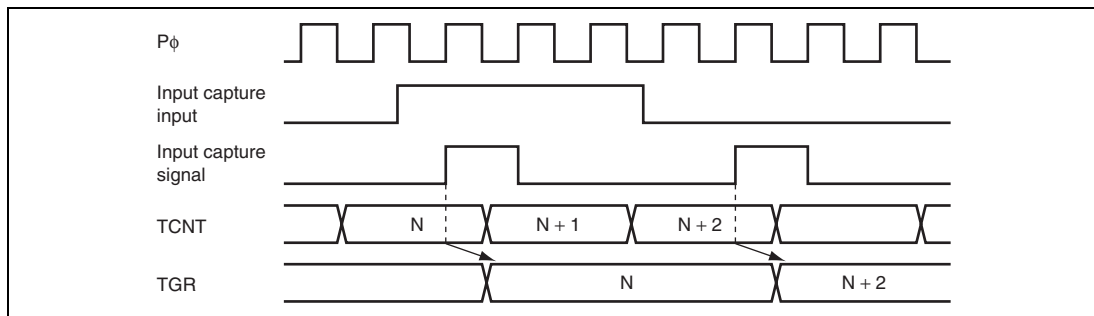
Figure 9.33 Input Capture Input Signal Timing
