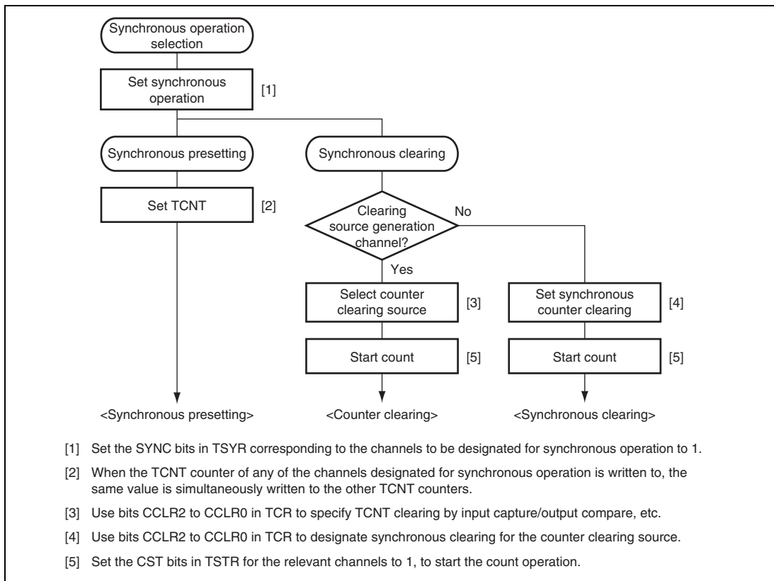
Figure 9.10 Example of Synchronous Operation Setting Procedure
