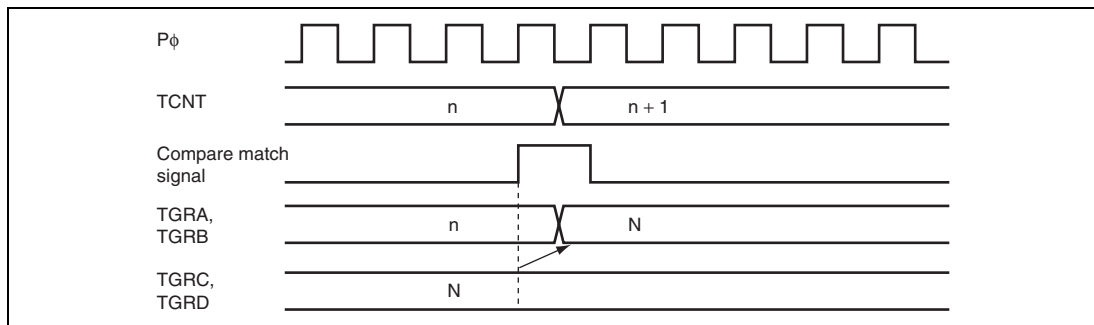
Figure 9.36 Buffer Operation Timing (Compare Match)
