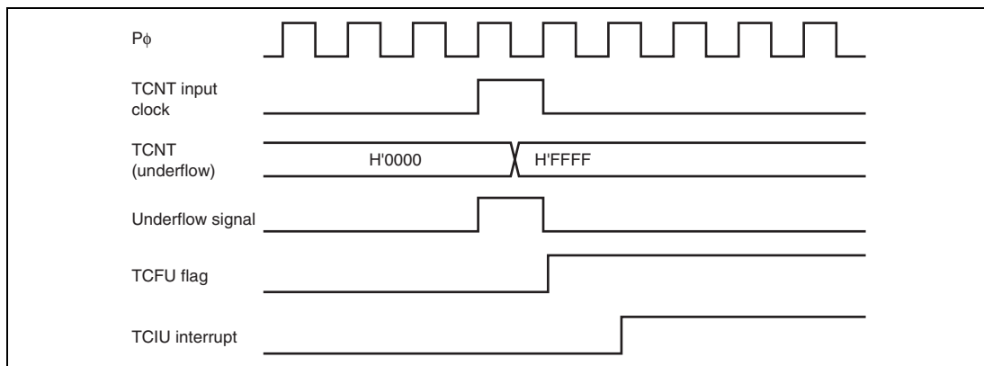
Figure 9.41 TCIU Interrupt Setting Timing
