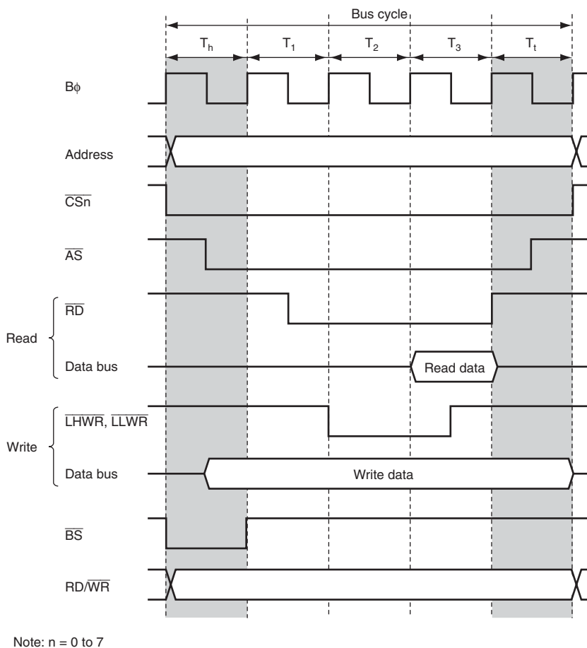
Figure 6.22 Example of Timing when Chip Select Assertion Period is Extended
