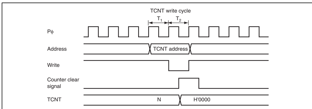
Figure 9.46 Conflict between TCNT Write and Clear Operations
