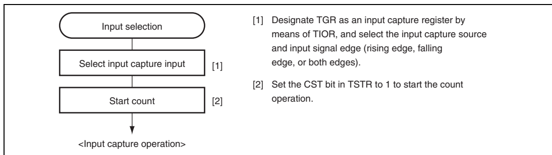
Figure 9.8 Example of Setting Procedure for Input Capture Operation
