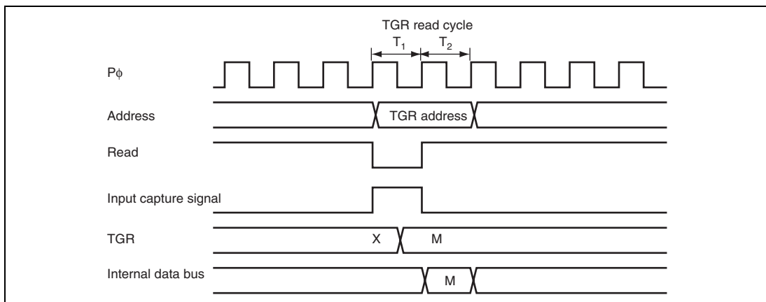
Figure 9.50 Conflict between TGR Read and Input Capture
