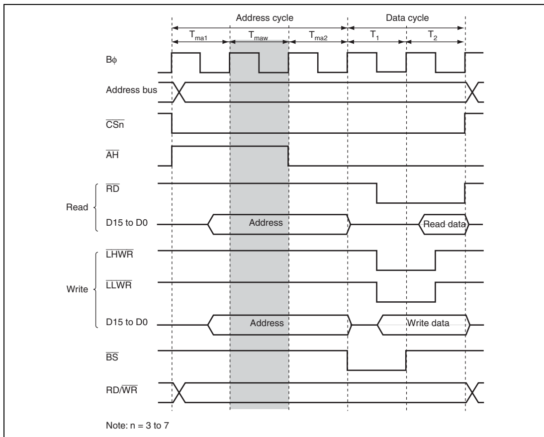
Figure 6.30 Access Timing of 3 Address Cycles (ADDEX = 1)
