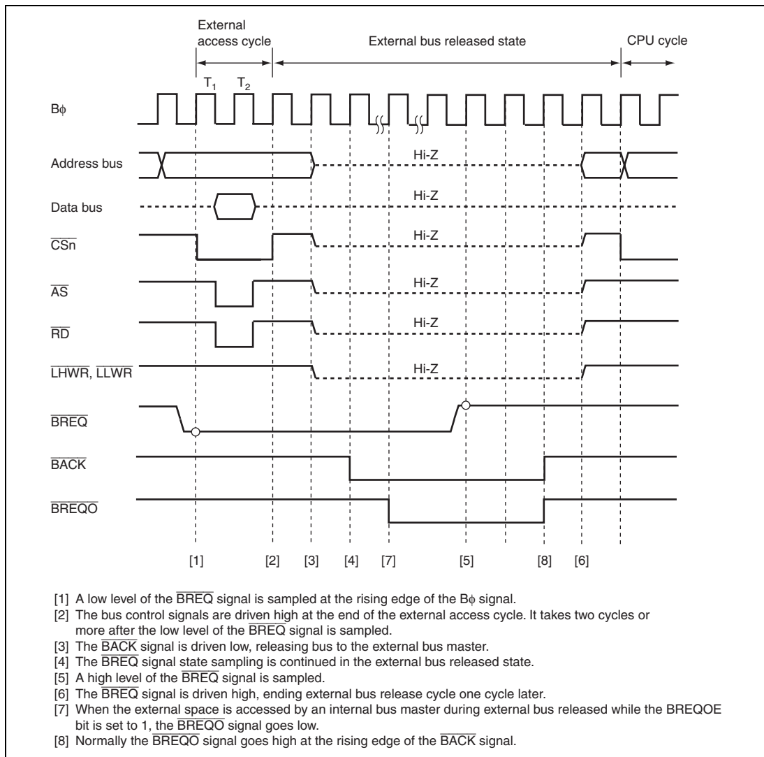
Figure 6.39 Bus Released State Transition Timing
