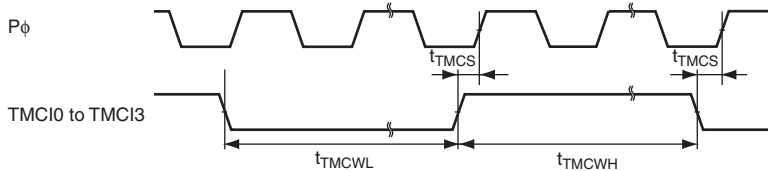
Figure 20.27 8-Bit Timer Clock Input Timing
