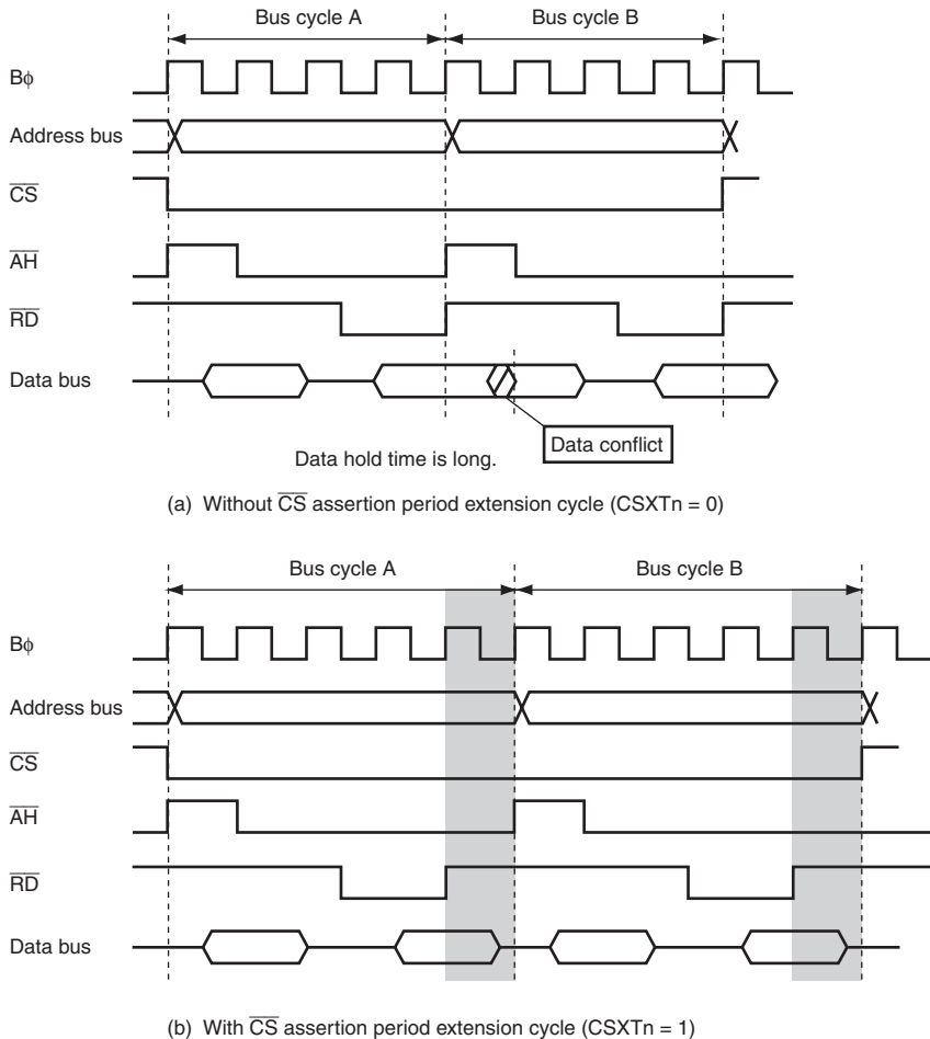
Figure 6.33 Consecutive Read Accesses to Same Area (Address/Data Multiplexed I/O Space)
