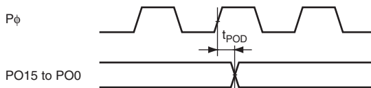
Figure 20.24 PPG Output Timing
