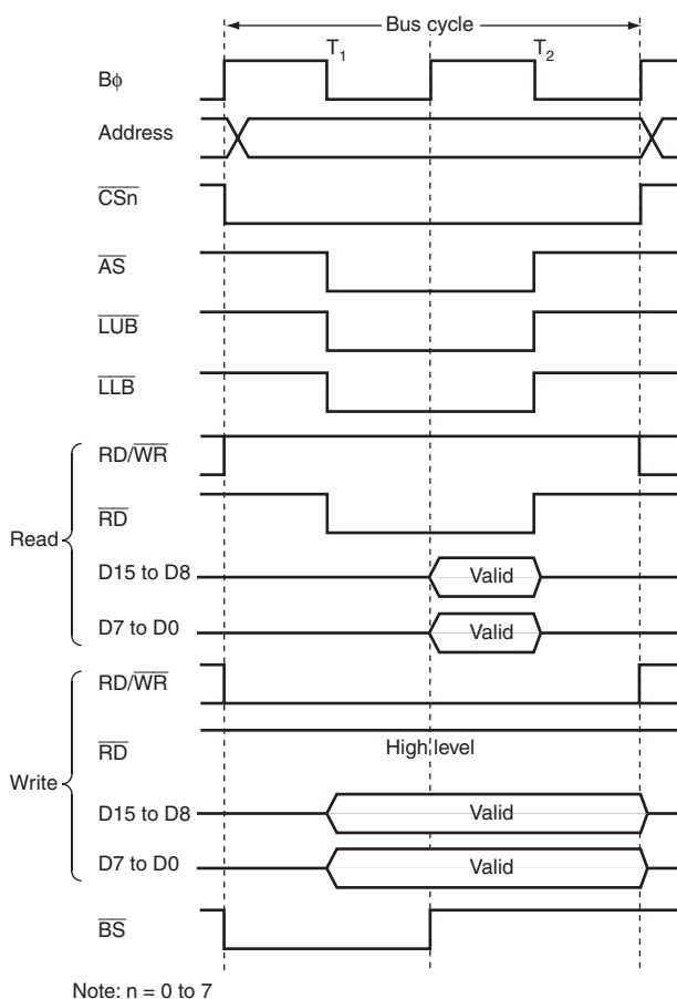
Figure 6.23 16-Bit 2-State Access Space Bus Timing
