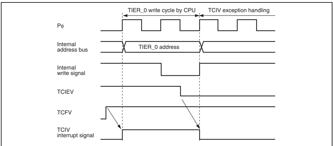
Figure 5.7 Conflict between Interrupt Generation and Disabling
