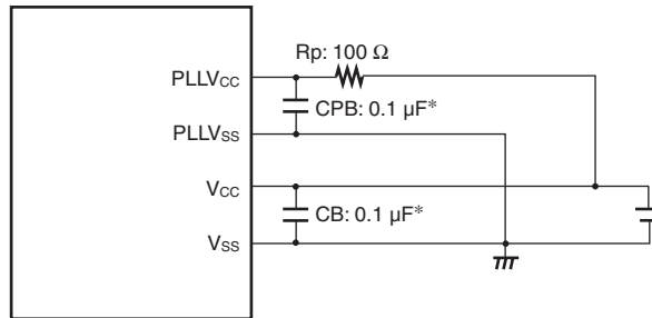
Figure 17.7 Recommended External Circuitry for PLL Circuit
