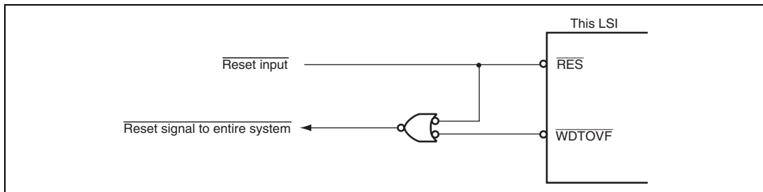
Figure 12.6 Circuit for System Reset by \overline{\text{WDTOVF}} Signal (Example)
