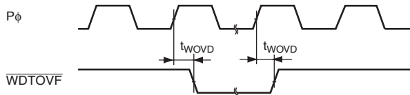
Figure 20.28 WDT Output Timing
