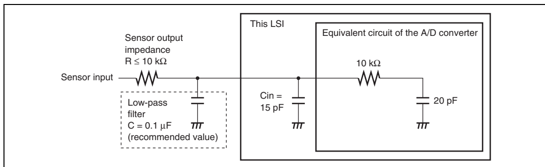
Figure 14.8 Example of Analog Input Circuit
