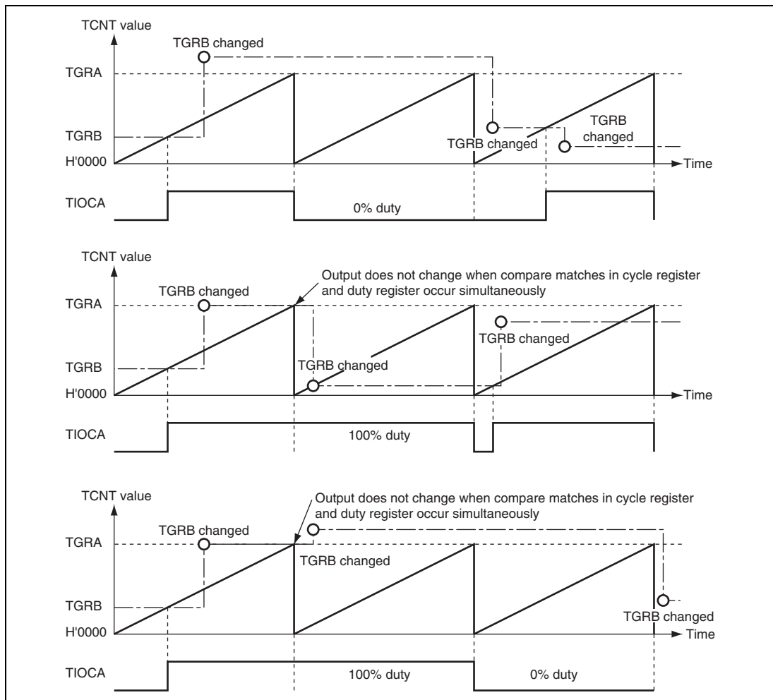
Figure 9.23 Example of PWM Mode Operation (3)
