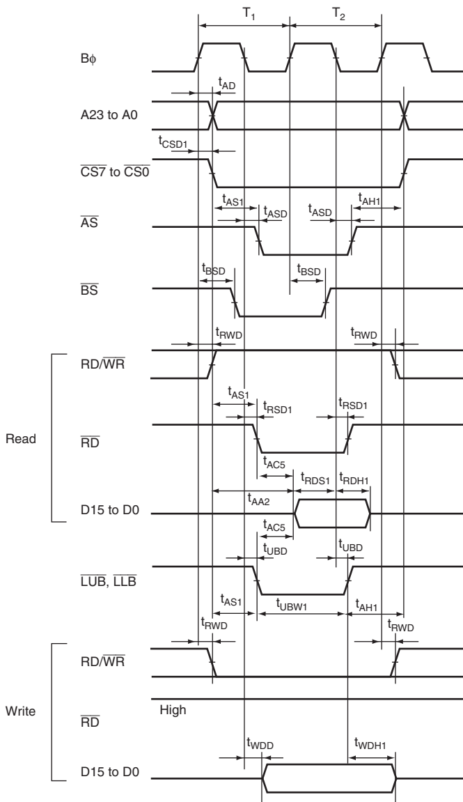
Figure 20.13 Byte Control SRAM: 2-State Read/Write Access
