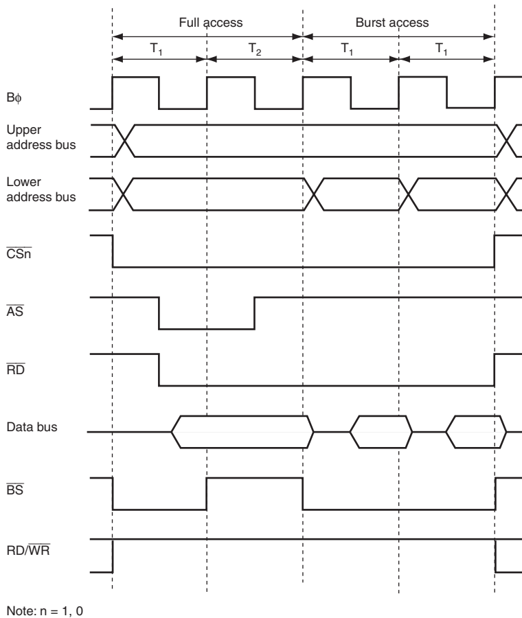
Figure 6.27 Example of Burst ROM Access Timing (ASTn = 0, One Burst Cycle)
