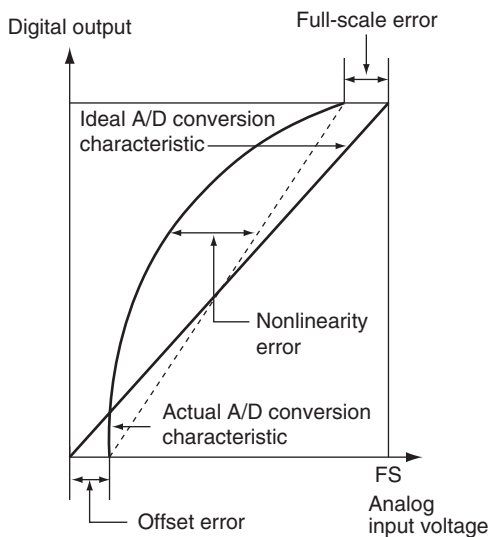
Figure 14.7 A/D Conversion Accuracy Definitions
