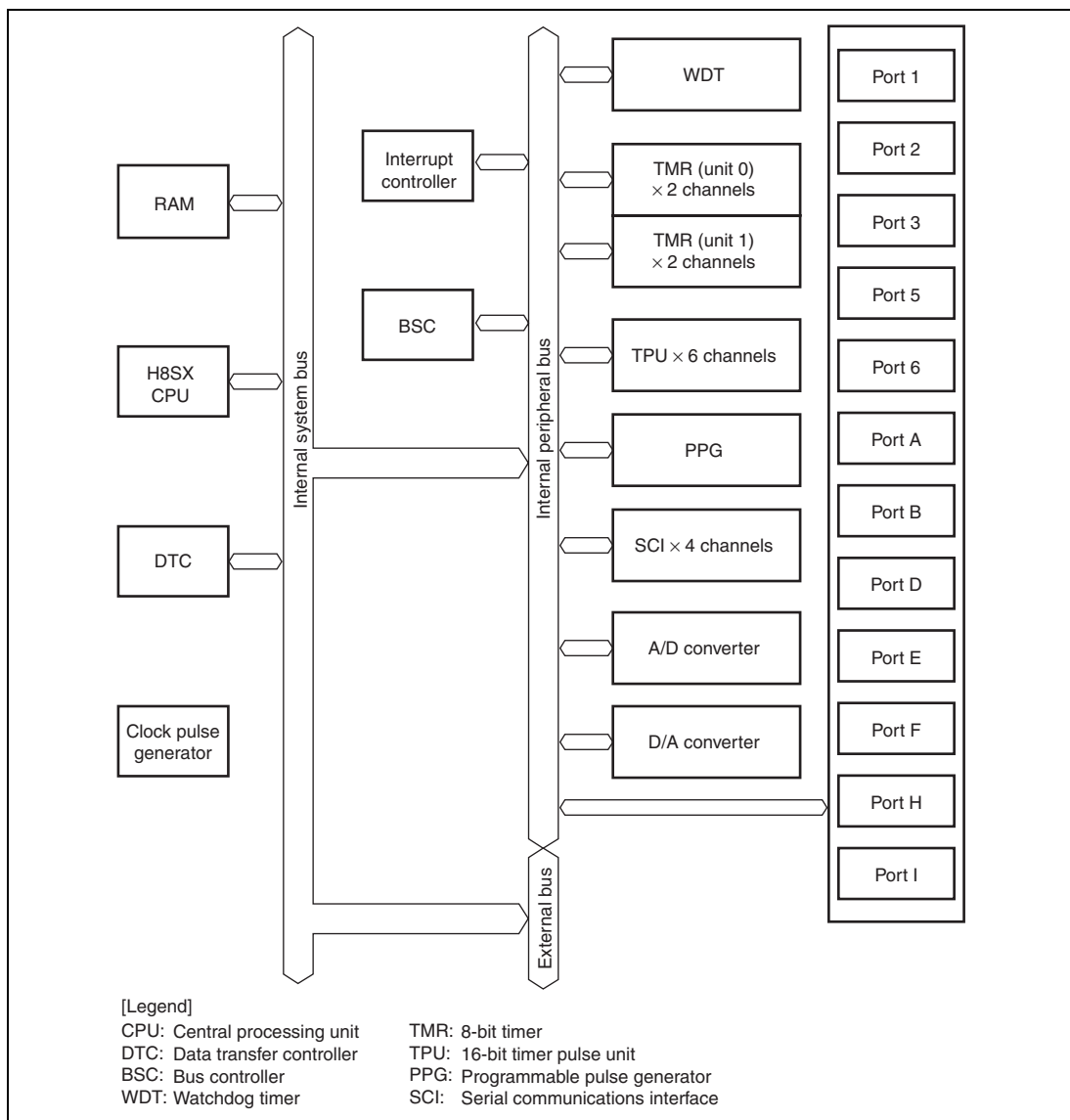
Figure 1.2 Block Diagram
