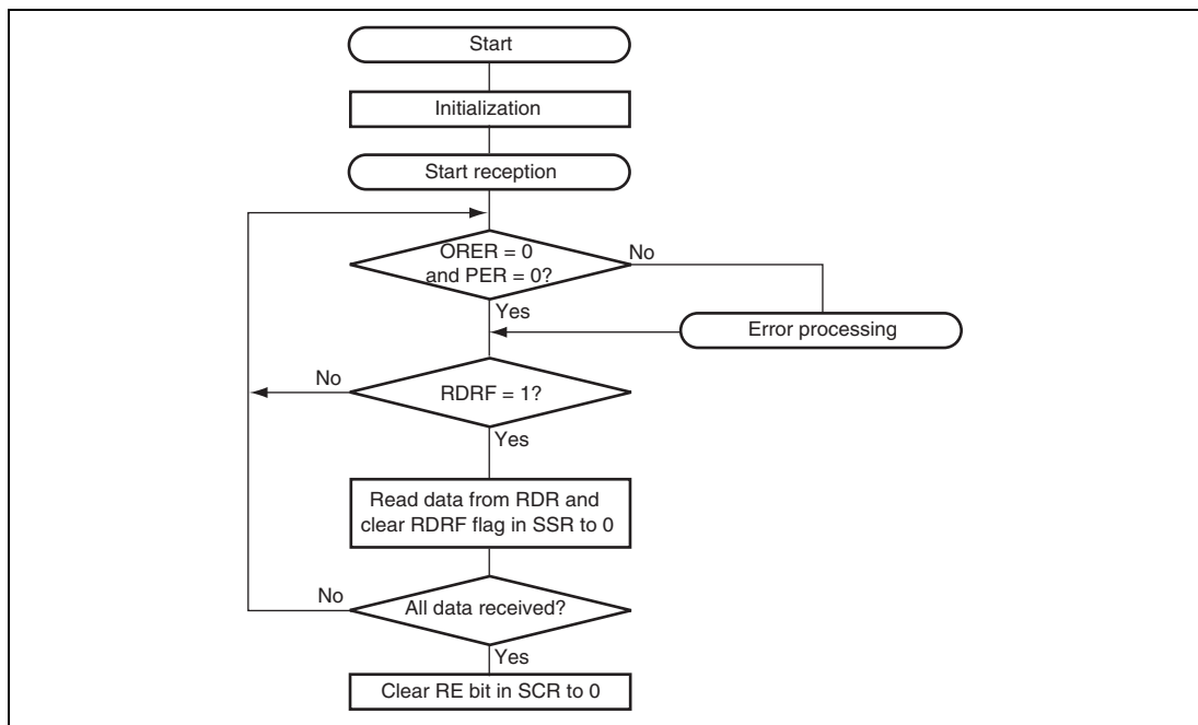
Figure 13.30 Sample Reception Flowchart
