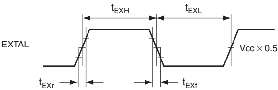
Figure 20.5 External Input Clock Timing
