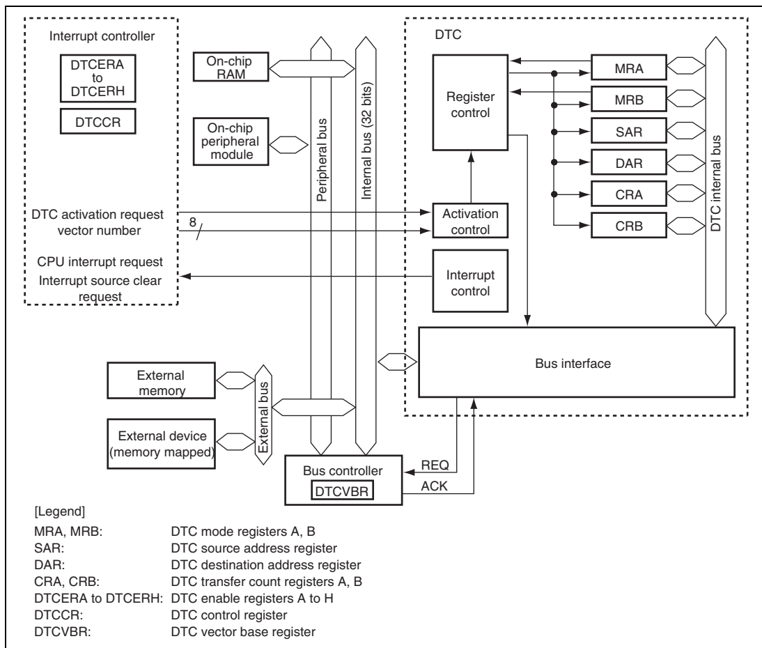
Figure 7.1 Block Diagram of DTC
