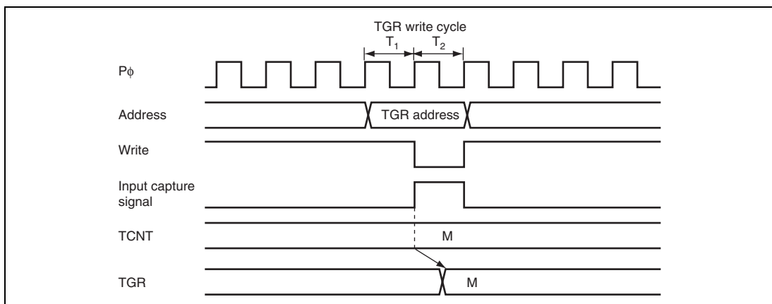
Figure 9.51 Conflict between TGR Write and Input Capture
