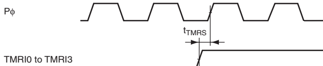
Figure 20.26 8-Bit Timer Reset Input Timing
