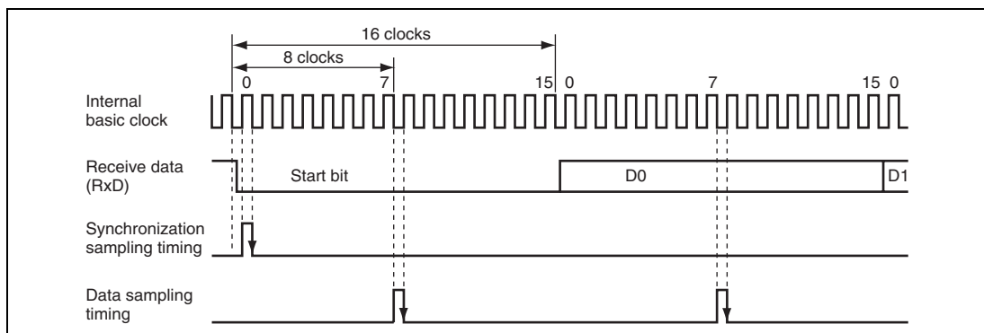
Figure 13.3 Receive Data Sampling Timing in Asynchronous Mode
