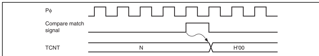
Figure 11.9 Timing of Counter Clear by Compare Match
