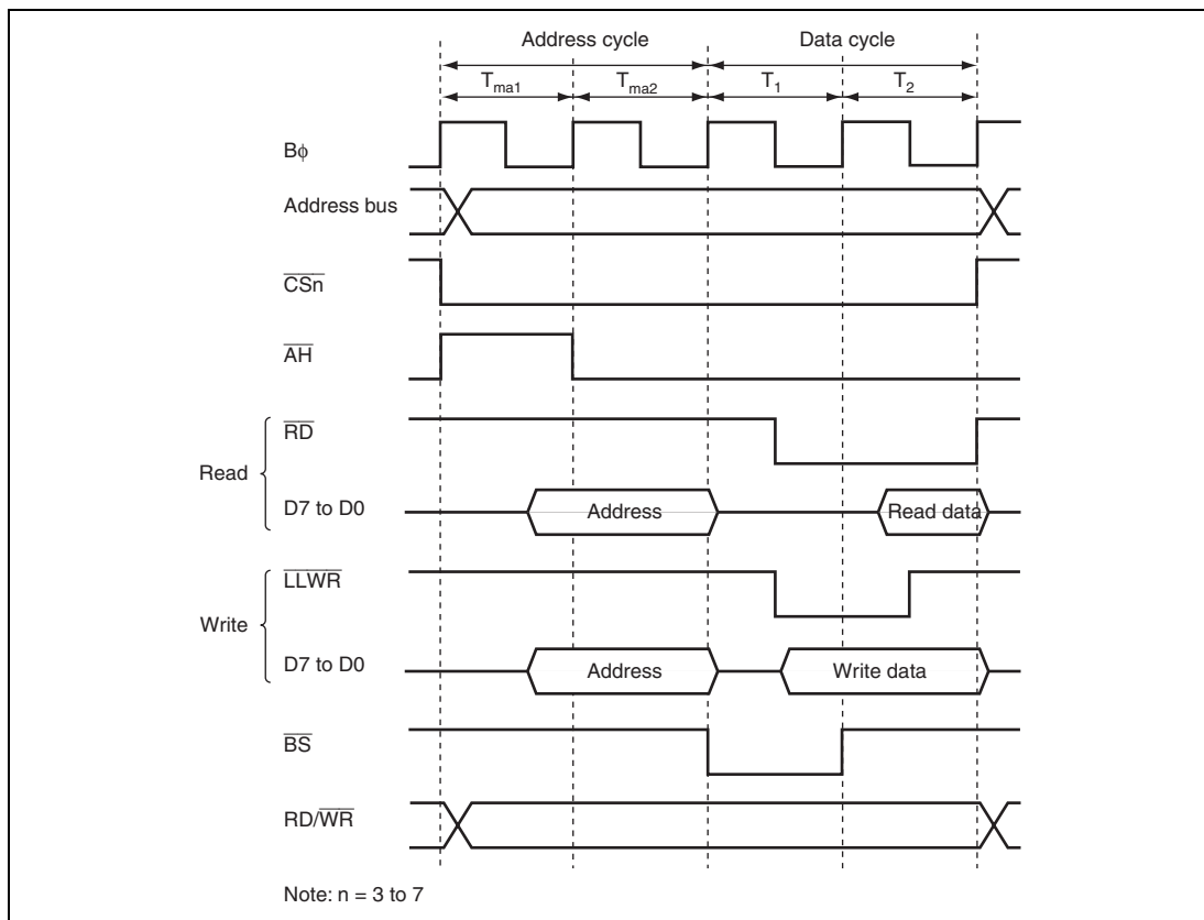
Figure 6.28 8-Bit Access Space Access Timing (ABWHn = 1, ABWLn = 1)
