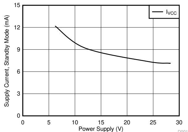
Figure 7-5. Supply Current vs Power Supply Voltage
