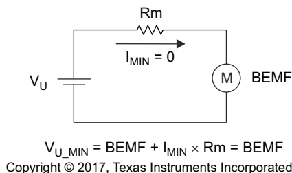
Figure 8-33. Mechanical AVS
