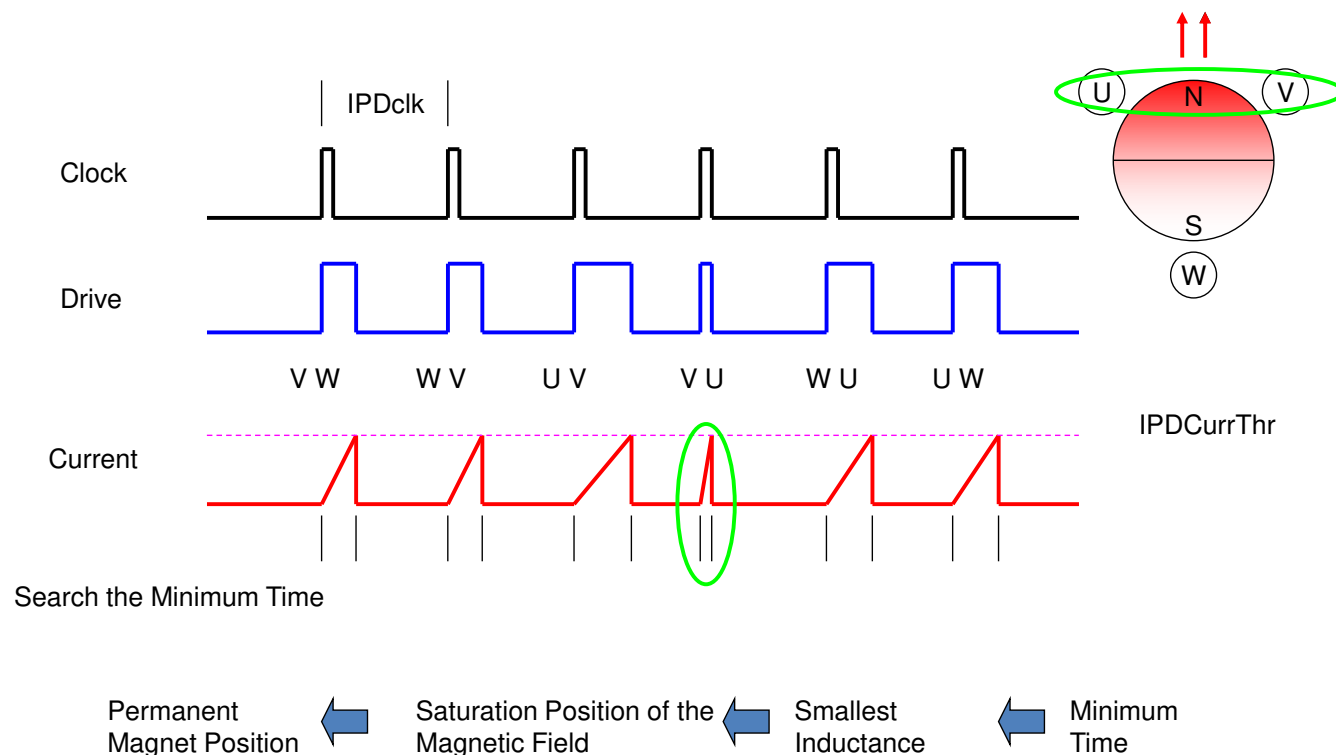
Figure 8-14. IPD Function
