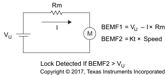
Figure 8-29. Lock Detection 1
