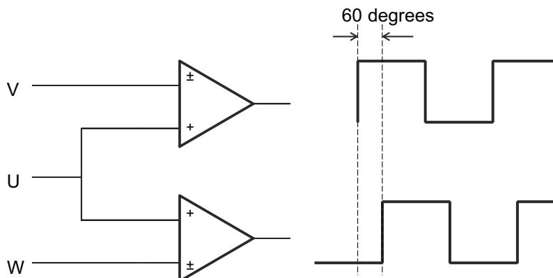
Figure 8-12. Initial Speed Detect Function
