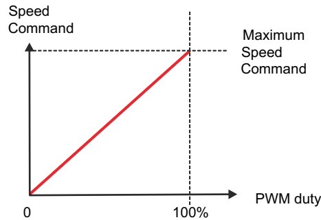
Figure 8-23. PWM-Mode Speed Command
