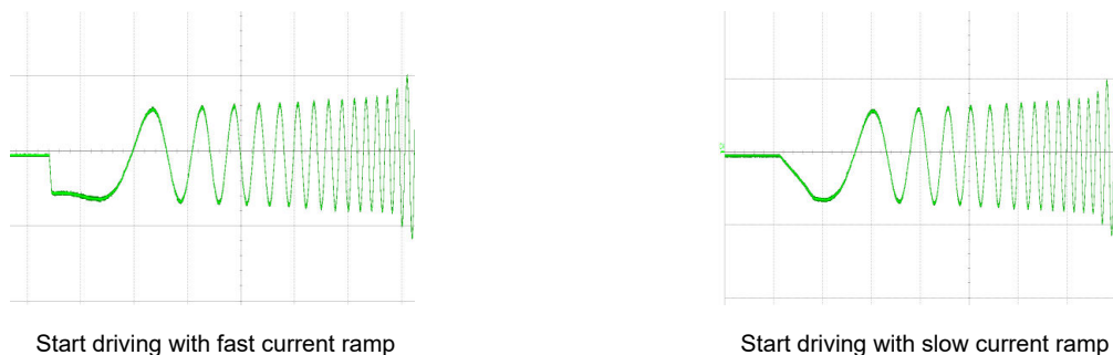
Figure 8-20. Motor Start-Up Current Ramp
