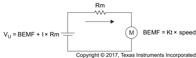
Figure 8-19. Motor Start-Up Current
