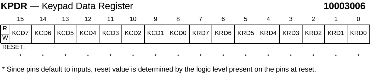
Figure C-20 Keypad Data Register
