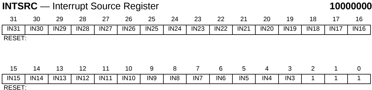
Figure C-1 Interrupt Source Register
