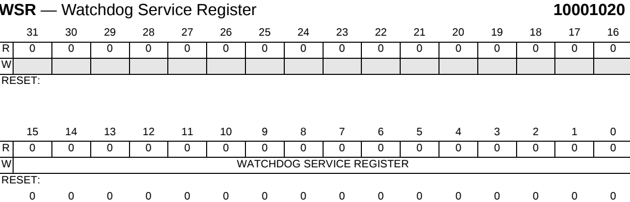
Figure 9-11 Watchdog Service Register
