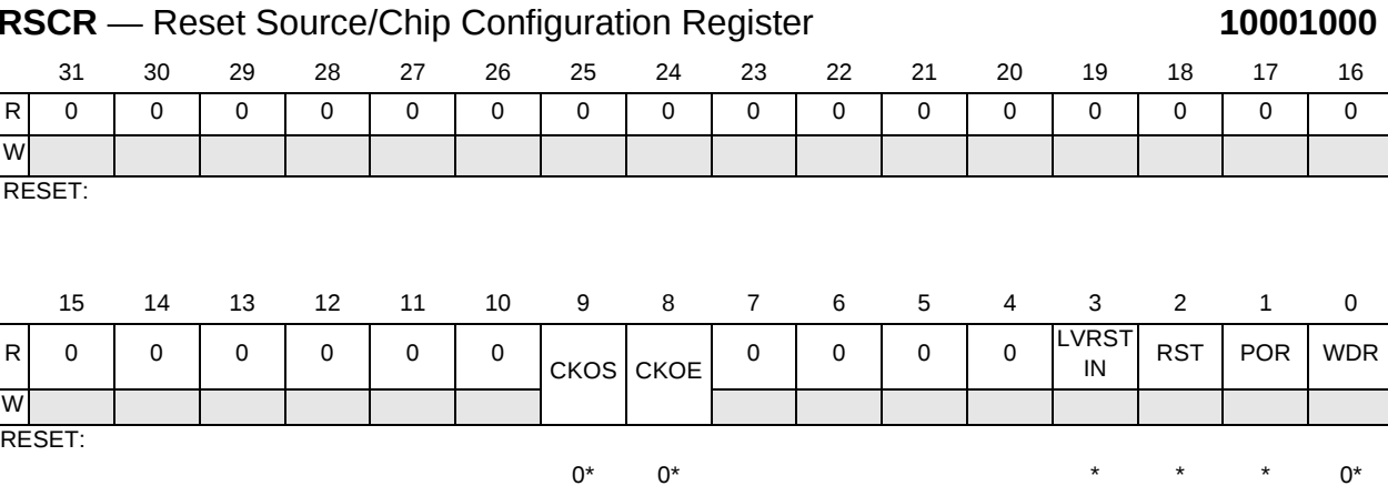
Figure 9-2 Reset Source Register
