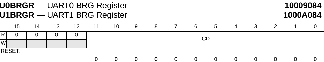
Figure 11-6 UART BRG Register
