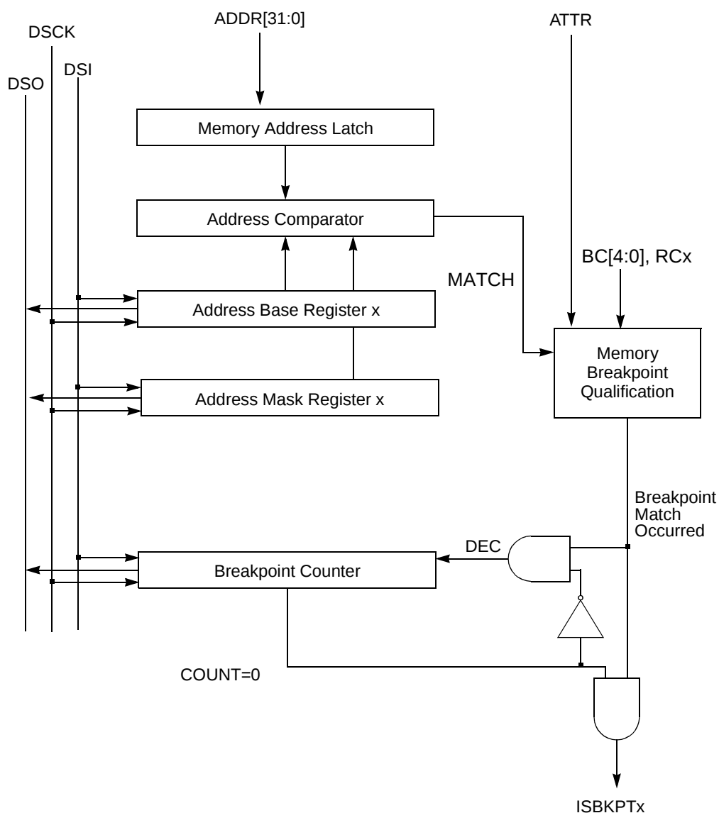
Figure 16-7 OnCE Memory Breakpoint Logic
