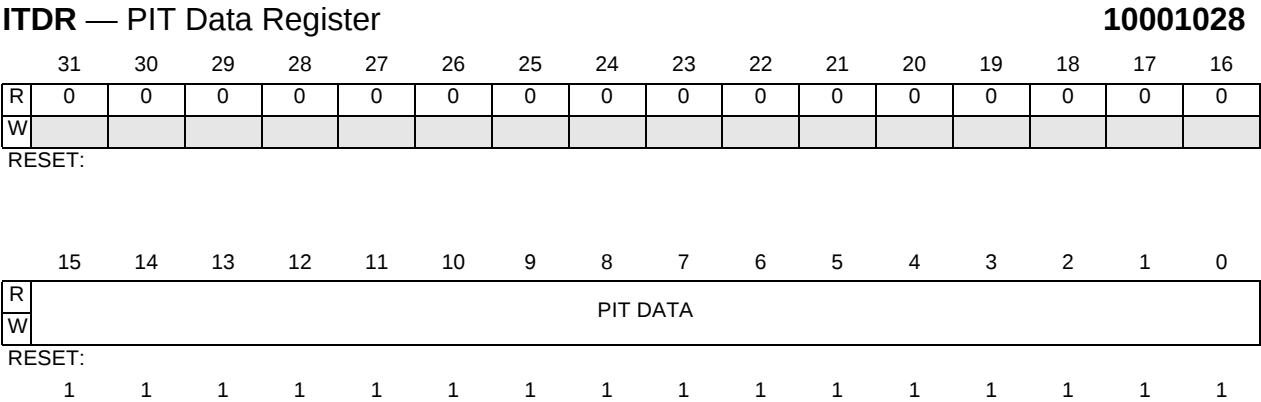
Figure C-15 PIT Data Register
