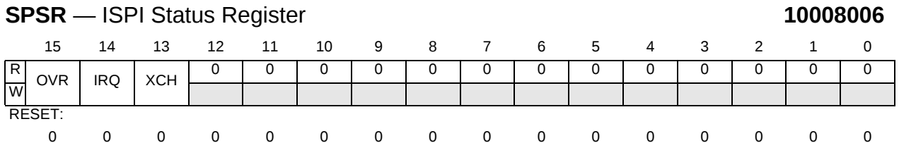
Figure 12-6 ISPI Status Register
