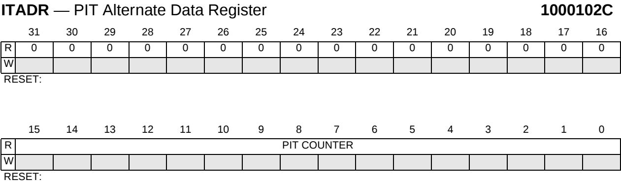
Figure C-16 PIT Alternate Data Register
