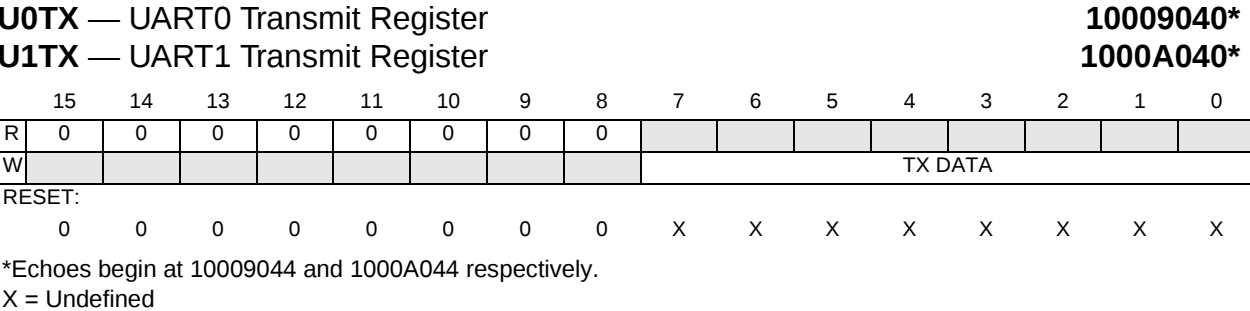
Figure C-37 UART Transmit Register
