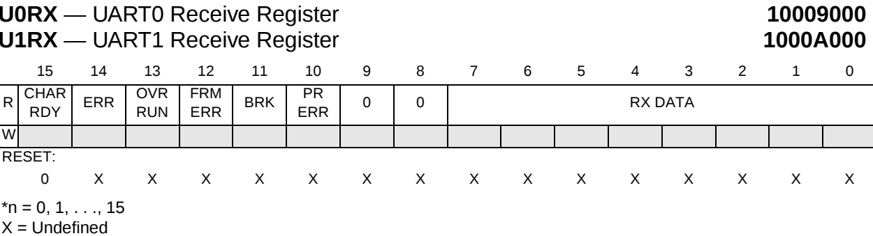
Figure 11-2 UART Receive Register
