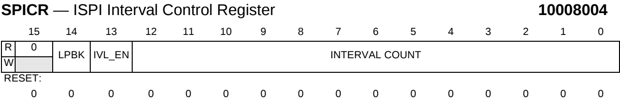
Figure 12-5 ISPI Interval Control Register
