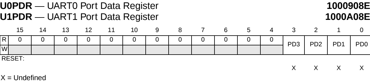
Figure 11-11 UART Port Data Register
