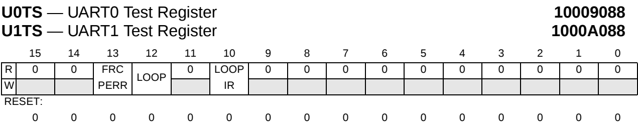
Figure 11-8 UART Test Register
