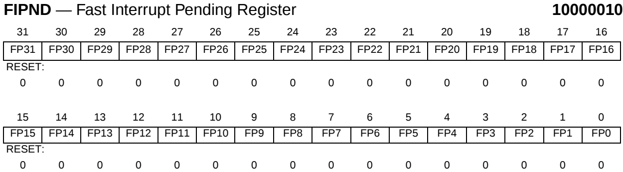
Figure 10-5 Fast Interrupt Pending Register
