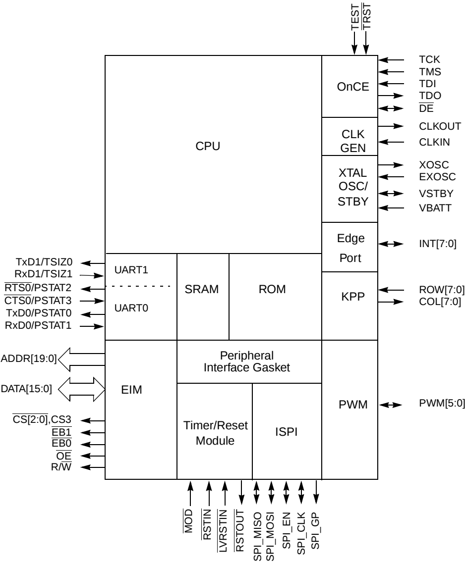
Figure 4-1 Functional Signal Groups
