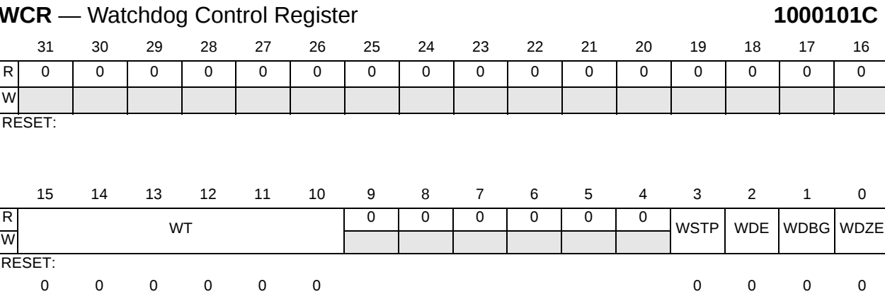
Figure 9-10 Watchdog Control Register
