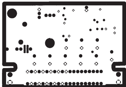
Figure 13. GND Layer
