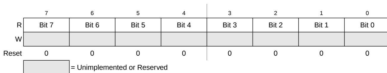
Figure 16-12. Debug Comparator C Register Low (DBG CCL)
